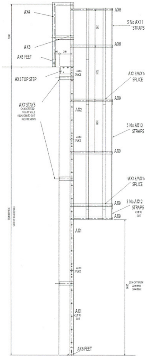
CUT DOWN AX1 LADDER SECTION AT BASE TO SUIT TYPICAL EXAMPLE FOR APPROX 5500mm RISE (5300 TO 6000 mm)
