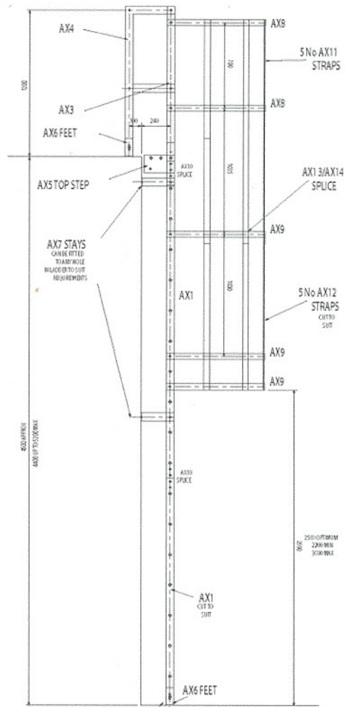
CUT DOWN AX1 LADDER SECTION AT BASE TO SUIT TYPICAL EXAMPLE FOR APPROX 4500mm RISE (4400 TO 5200 mm)
