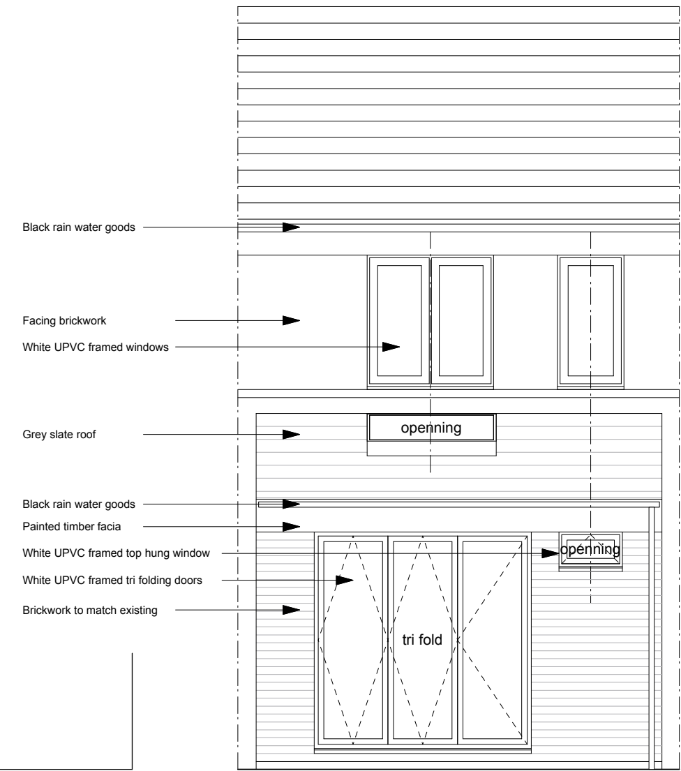
Rear Elevation
