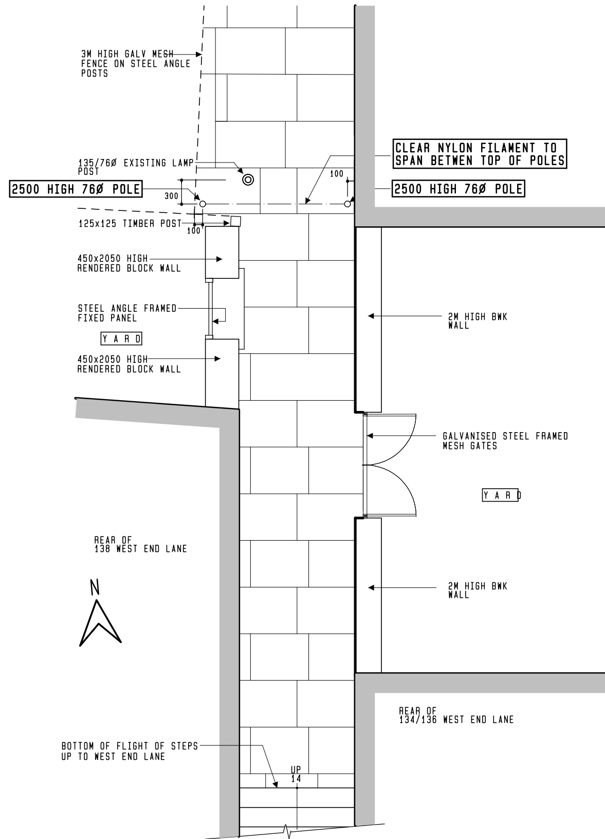
1:50 PLAN SHOWING LOCATION OF ERUV POLES WITH CLEAR NYLON FILAMENT BETWEEN
