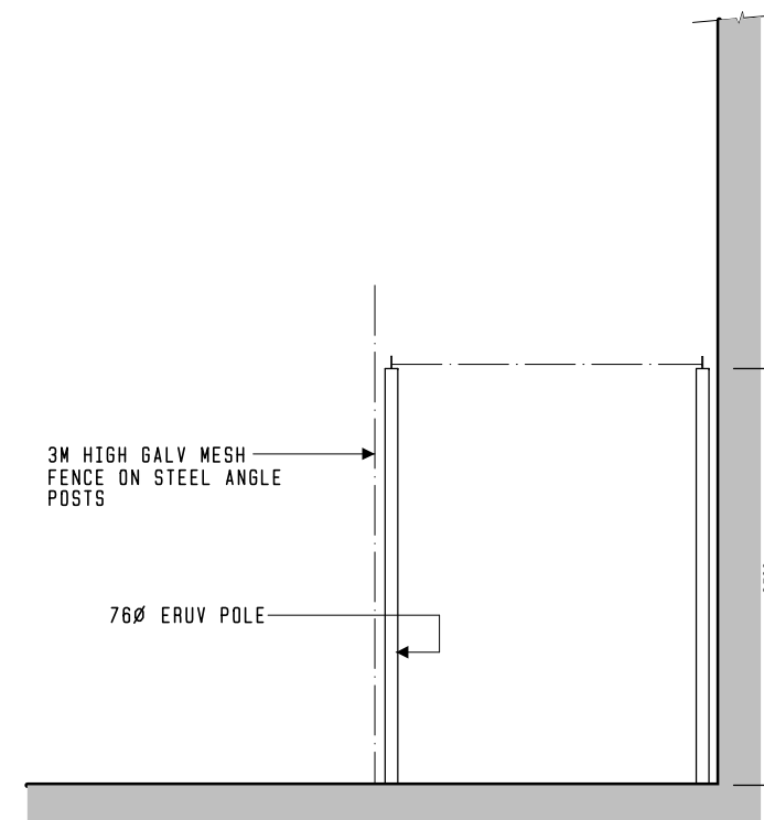
1:50 ELEVATION OF POLES AND CLEAR NYLON FILAMENT
