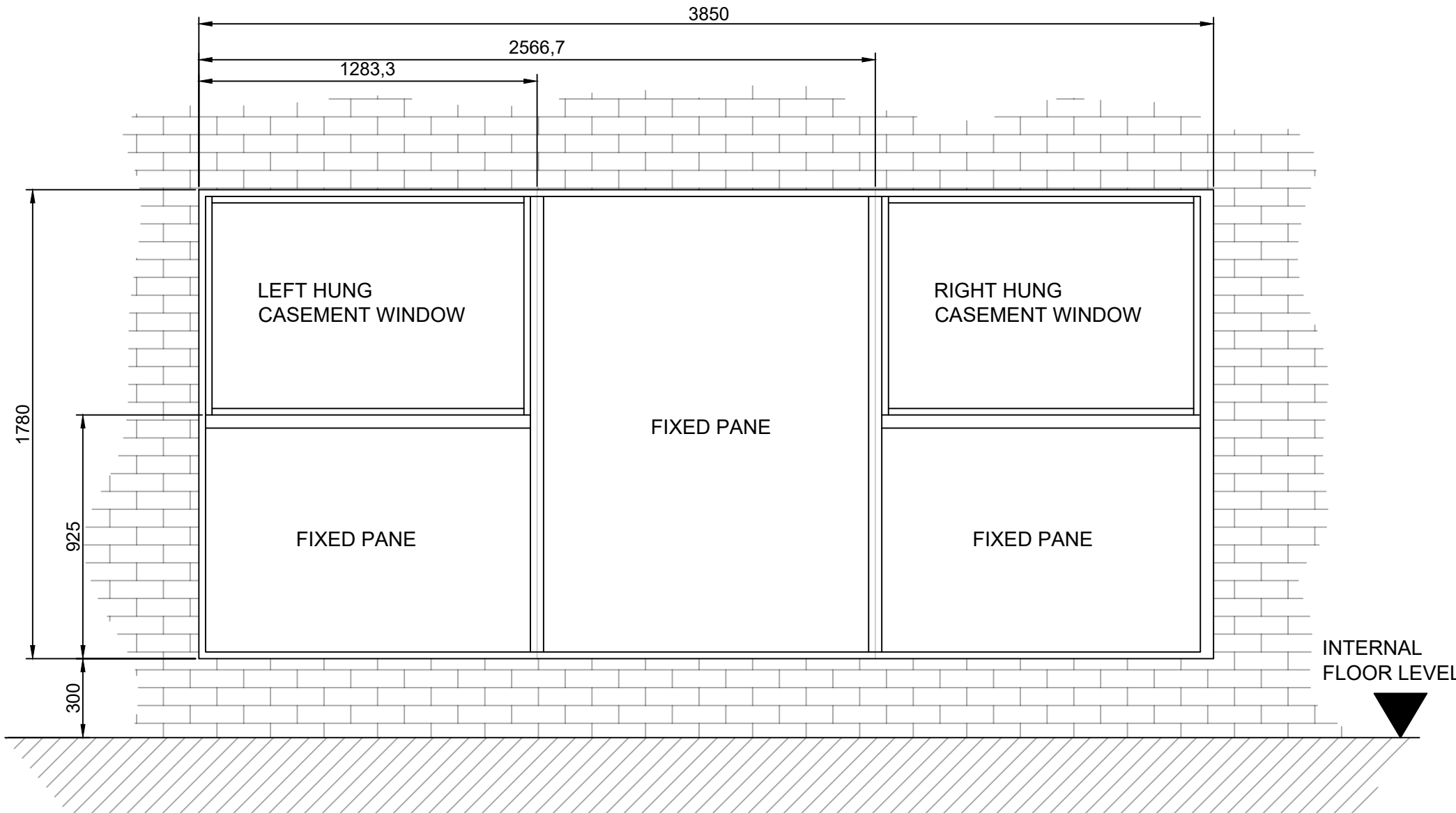
1 FRONT VIEW 1:20 @ A4
