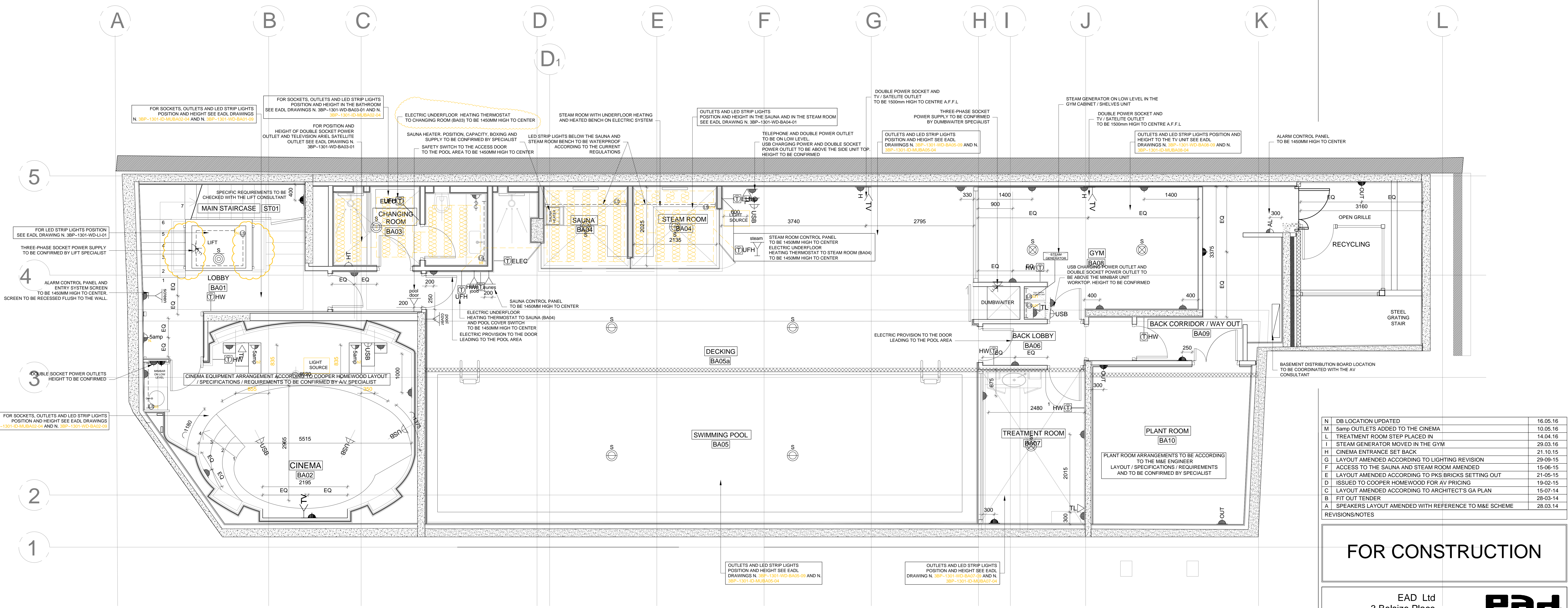
1 BASEMENT FLOOR PLAN - ELECTRIC LAYOUT SCALE:1:50 @ A1
