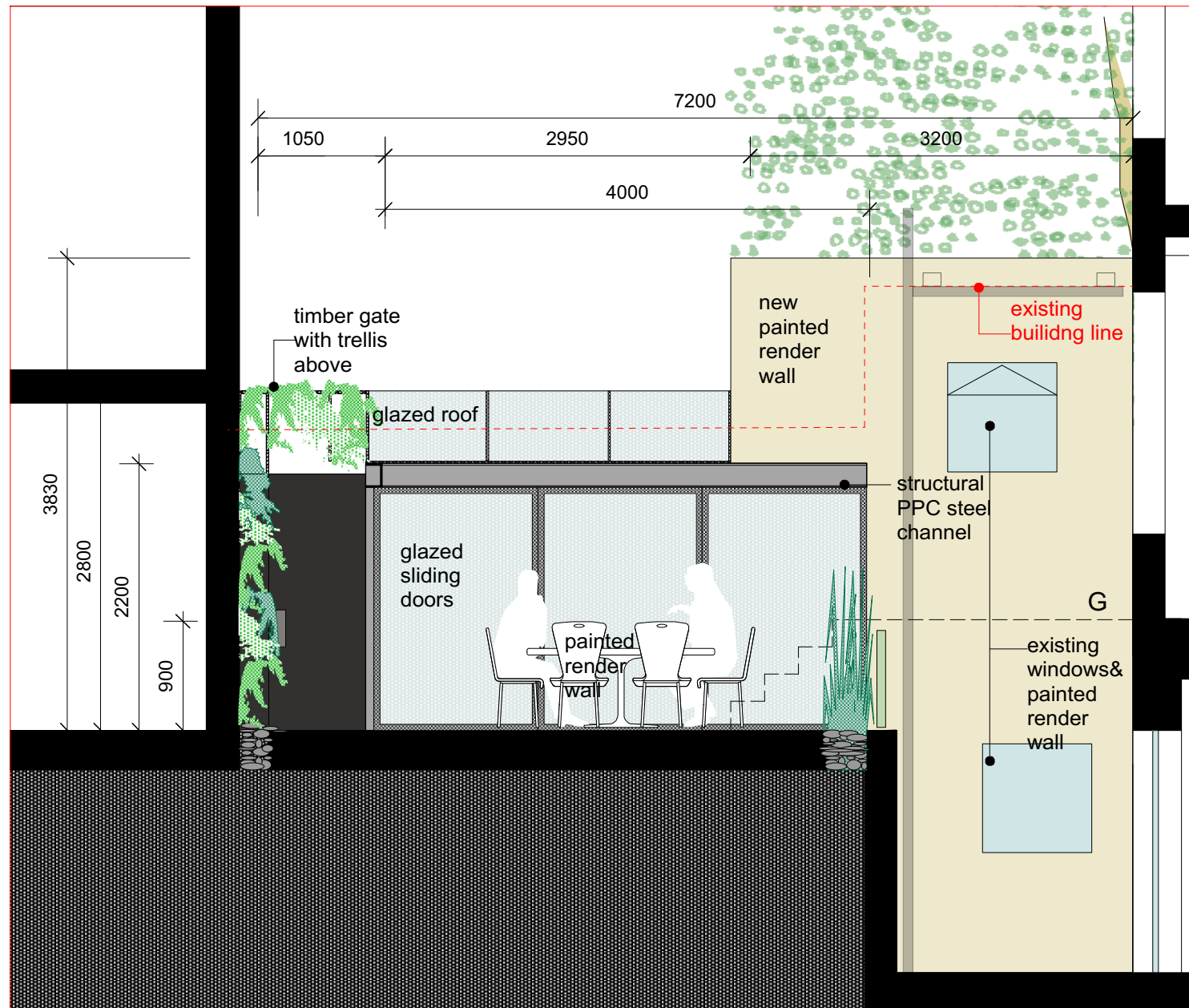
(A/2.25) SECTION NORTH-SOUTH scale 1:50
