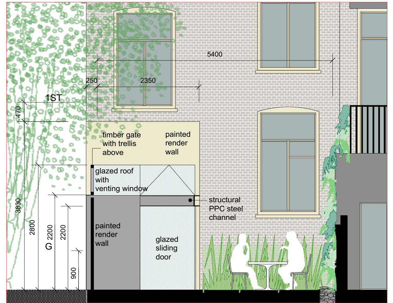
(EE/2.23) SECTION SOUTH-NORTH scale 1:50
