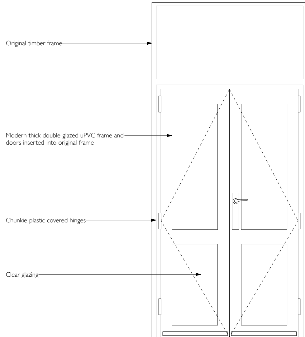
A EXISTING - French door elevation Scale 1-50
