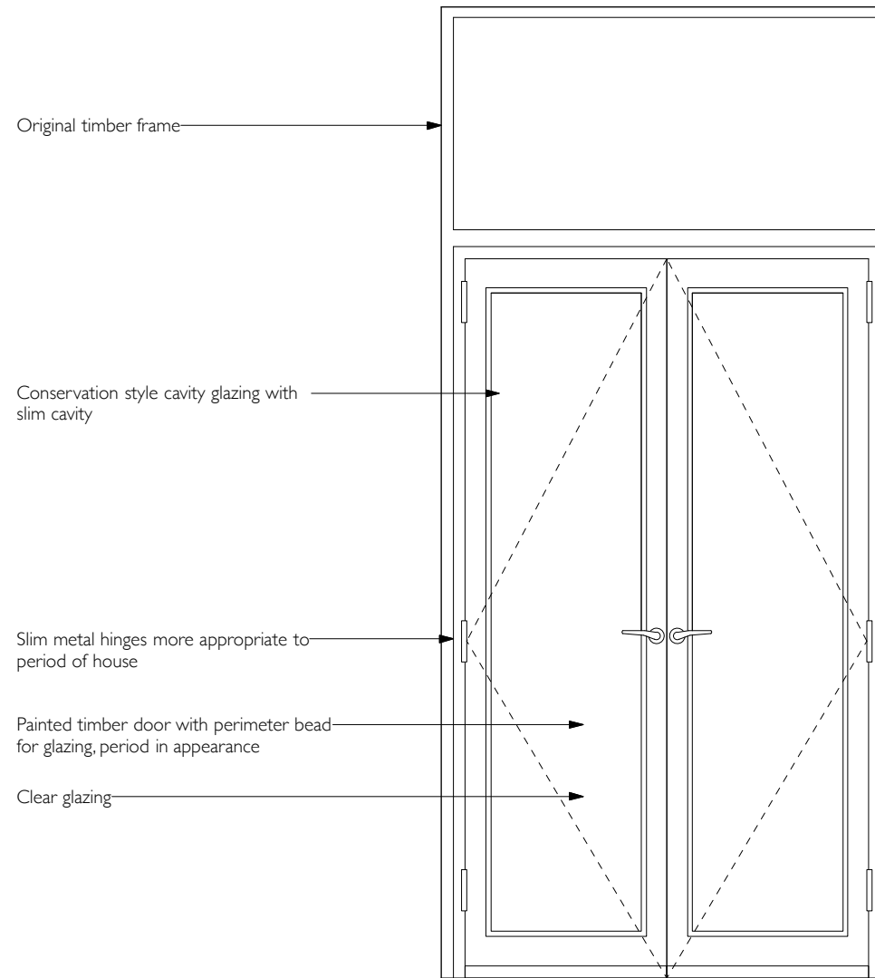
B PROPOSED - French door elevation Scale 1-50
