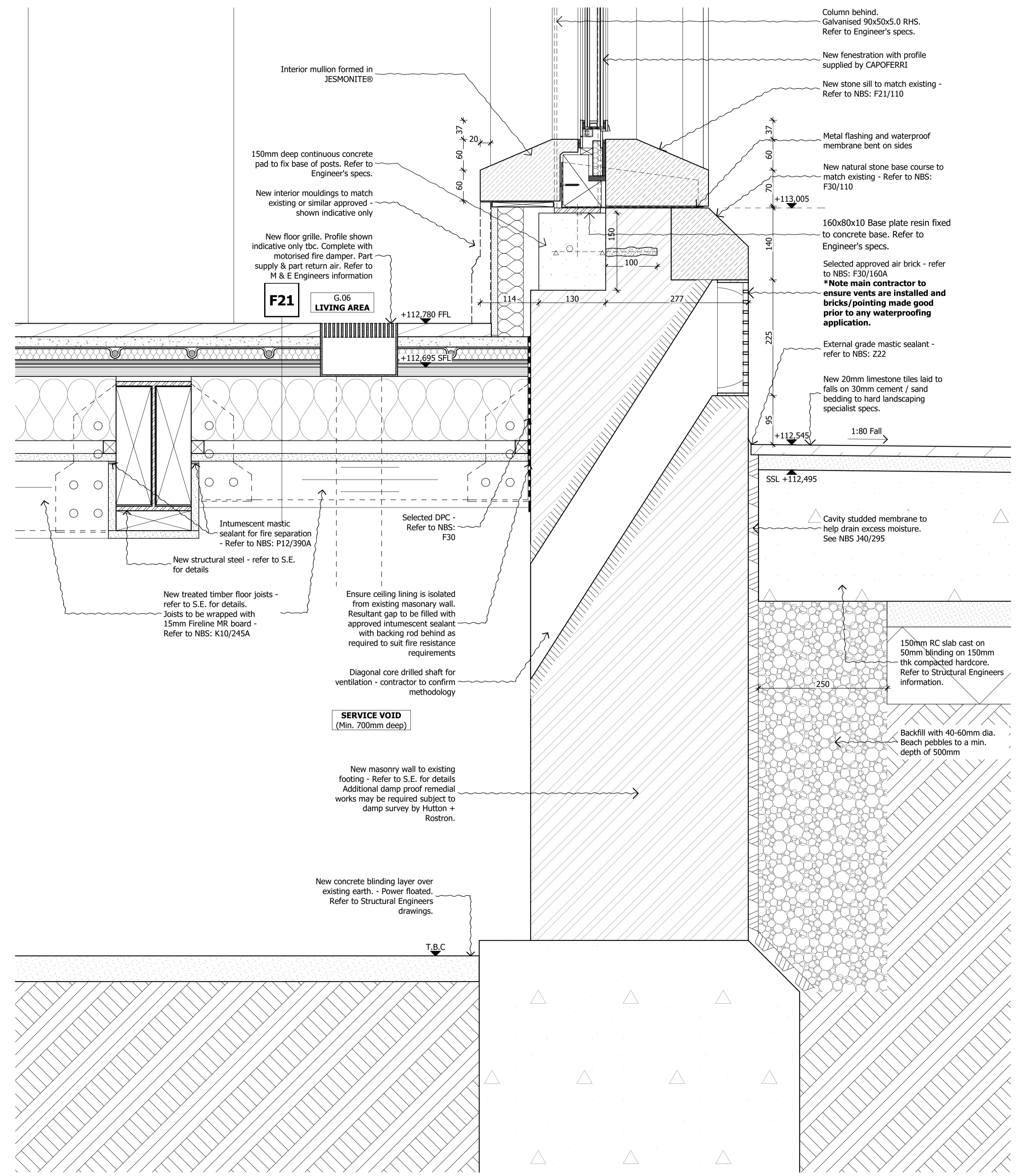
2 SCALE 1:5 @ A1; 1:10 @ A3 SECTION D-D DETAIL - NEW BAY WINDOW SILL AND BELOW GROUND
