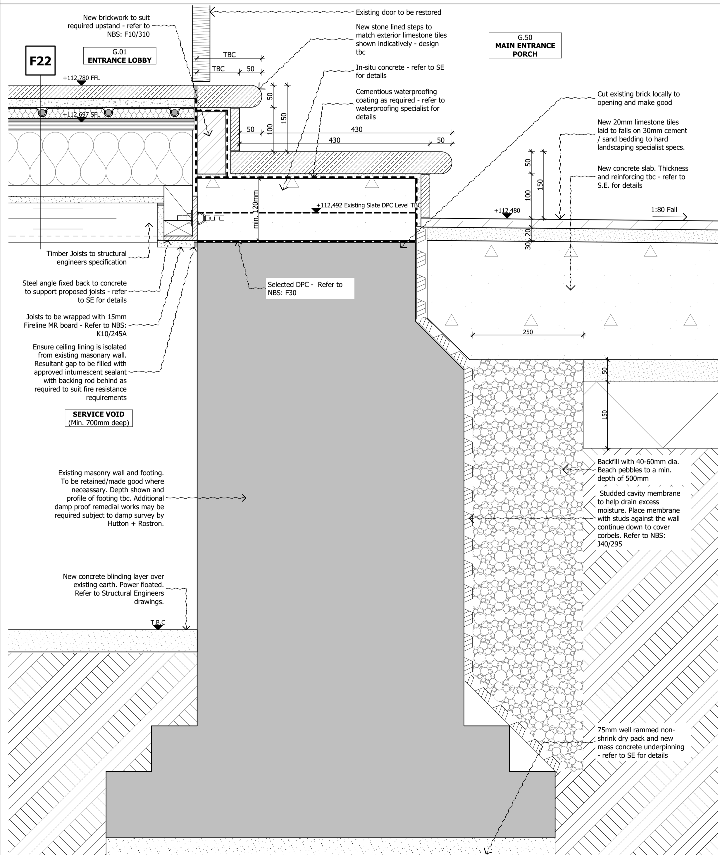
1 SCALE 1:5 @ A1; 1:10 @ A3 SECTION B-B DETAIL - GROUND FLOOR MAIN DOOR THRESHOLD IN EXISTING WALL
