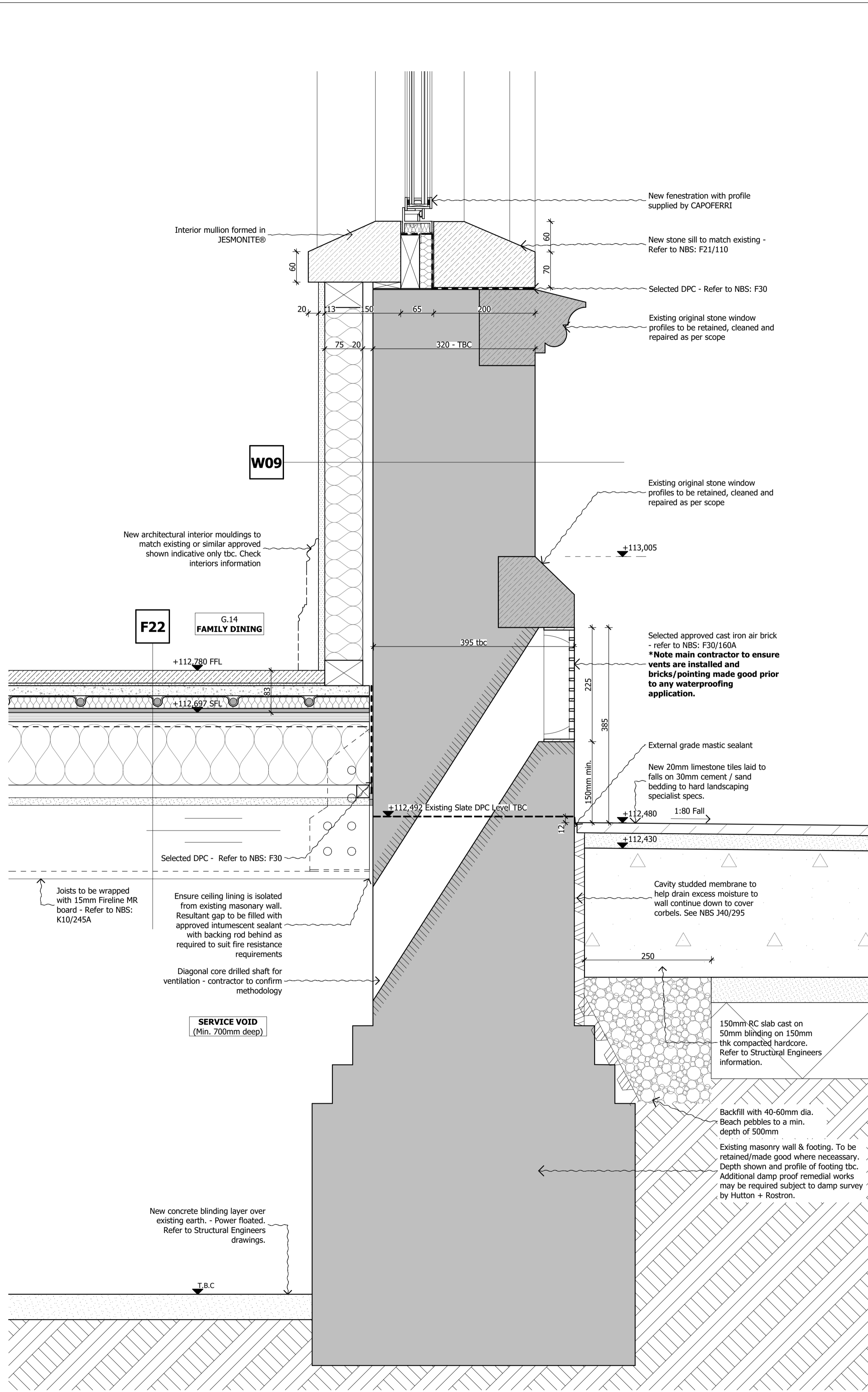
2 SCALE 1:5 @ A1; 1:10 @ A3 SECTION C-C DETAIL - GROUND FLOOR WINDOW SILL WITH VENT TO SOLUM
