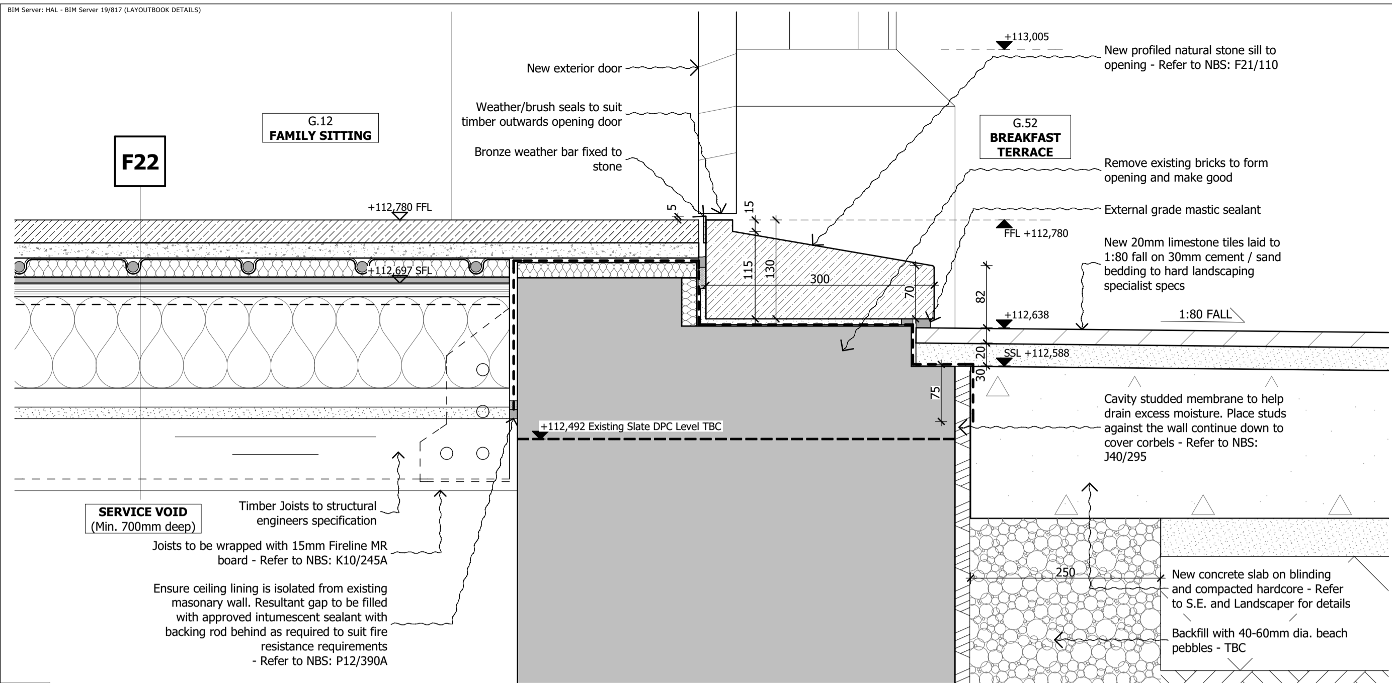
3 SCALE 1:5 @ A1; 1:10 @ A3 SECTION DETAIL - FAMILY SITTING DOOR THRESHOLD
