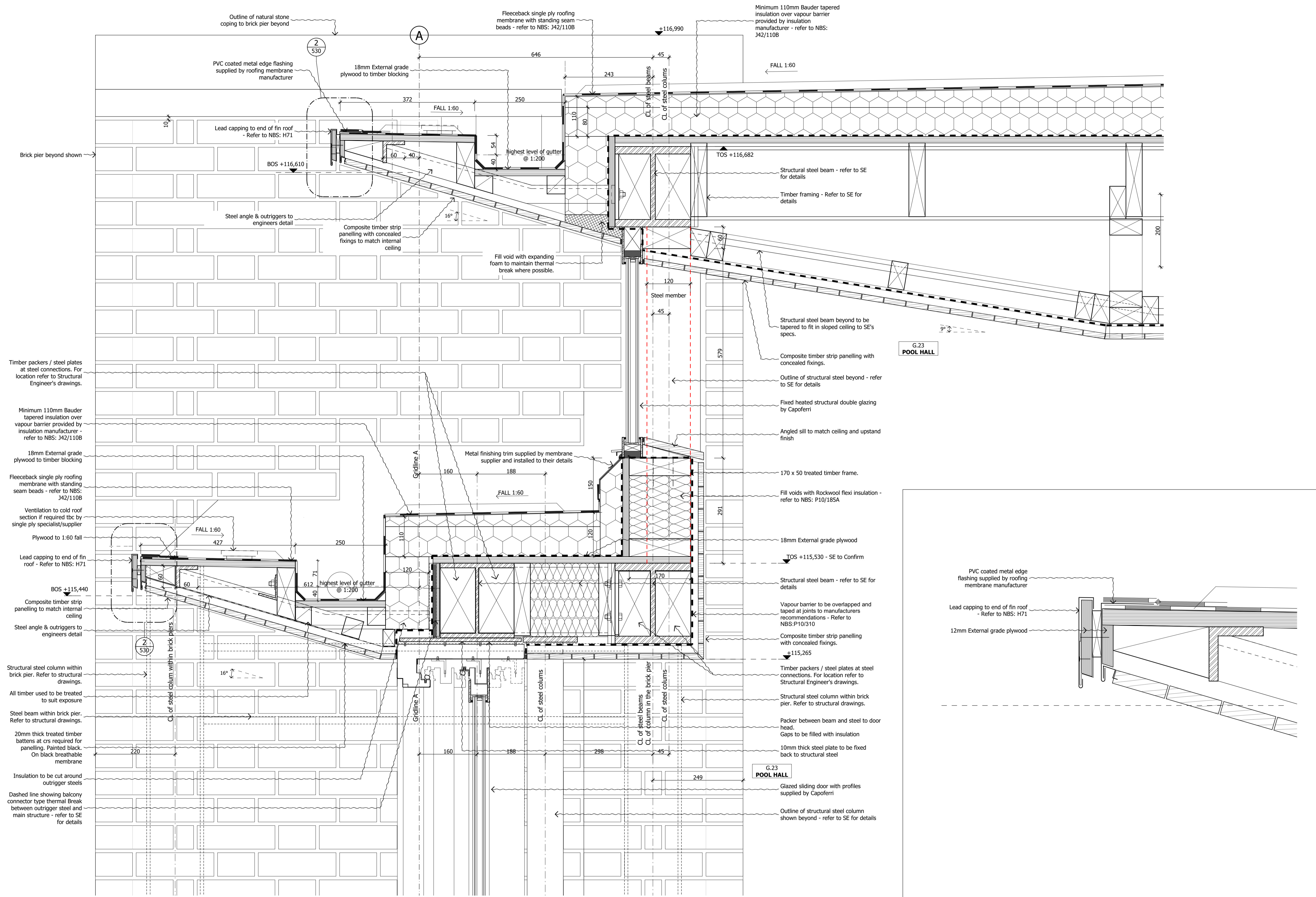
1 SCALE 1:5 @ A1; 1:10 @ A3 FLOORING ROOF DETAIL
