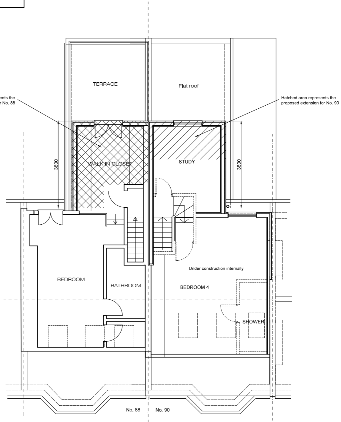
PROPOSED LOFT PLAN
