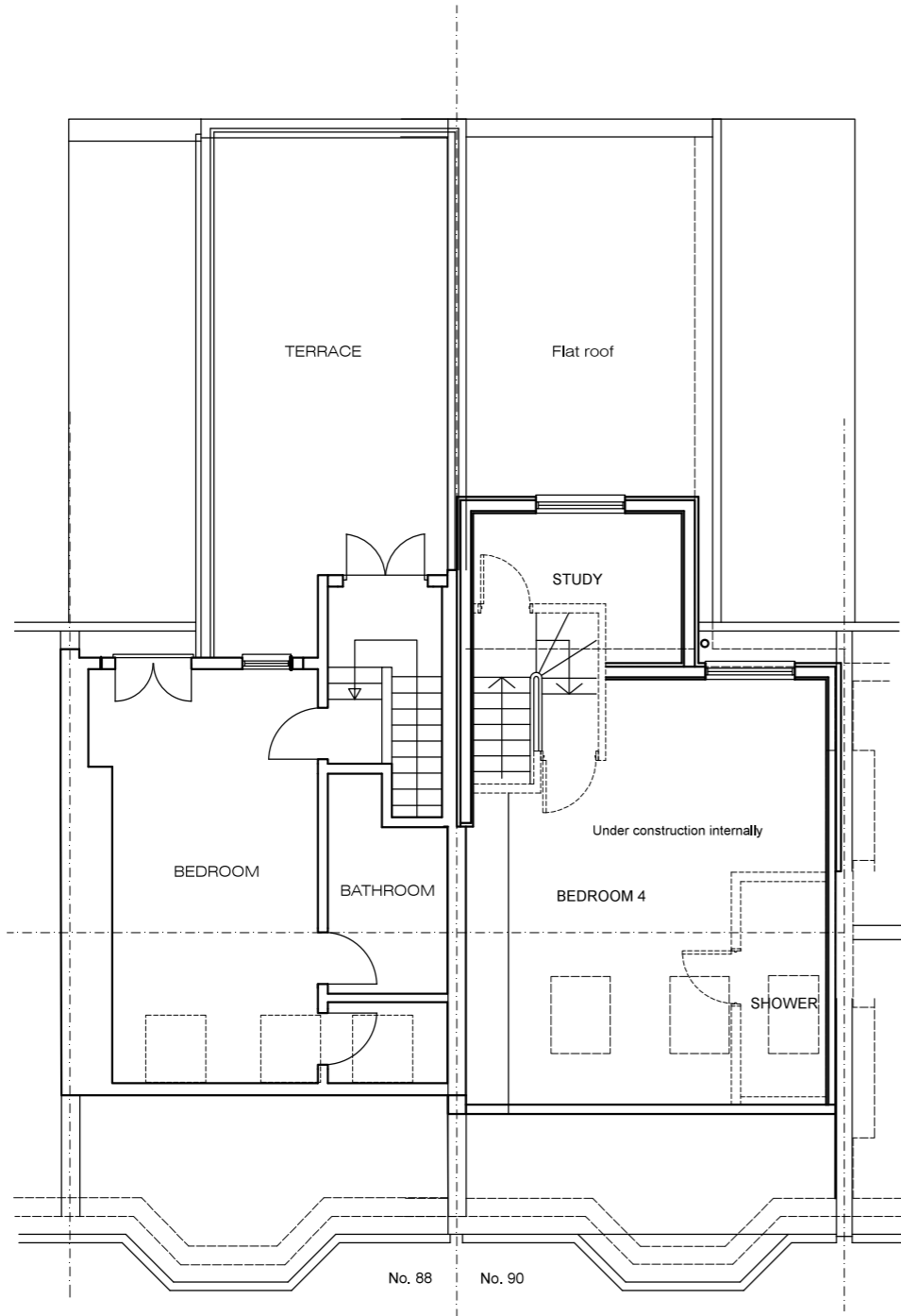
0m 1m 3m EXISTING LOFT PLAN
