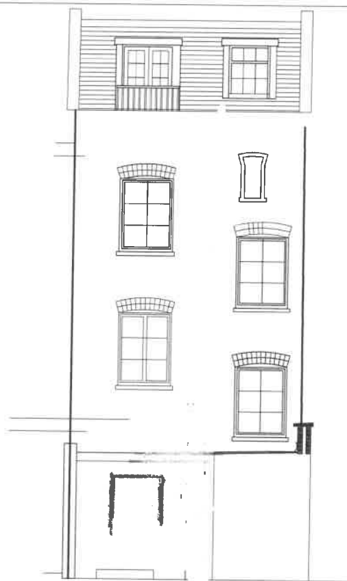
EXISTING REAR ELEVATION / SECTION
