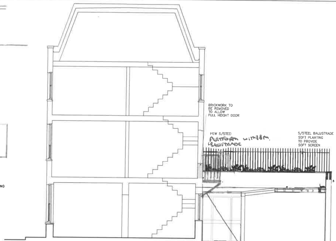
PROPOSED SECTION
