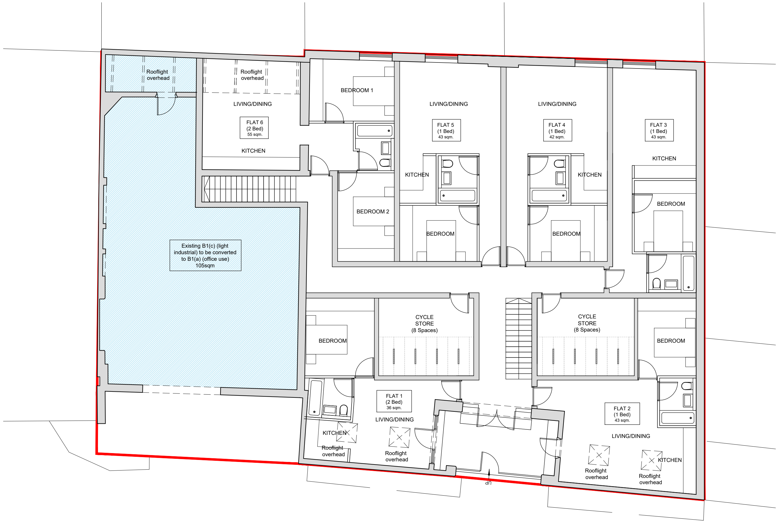
PROPOSED GROUND FLOOR PLAN SCALE 1:100
