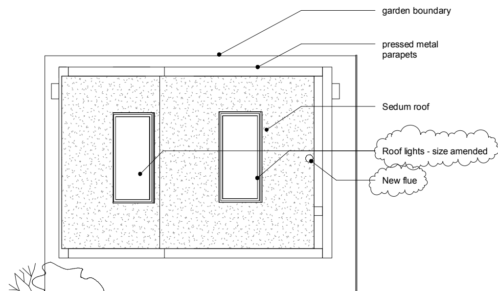
5 Garden Room Proposed Plan 1 : 100
