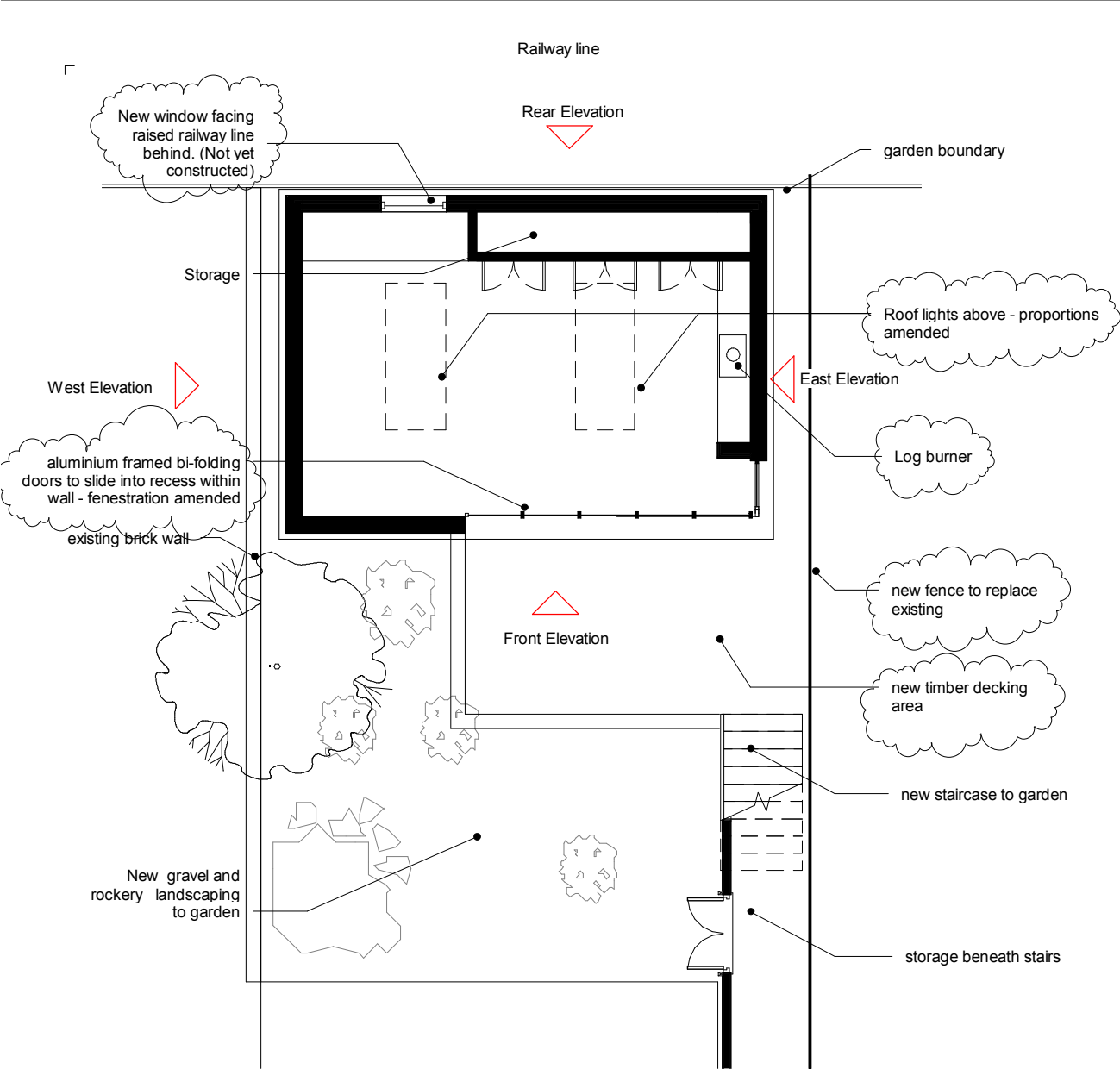
5 Garden Room Proposed Plan 1 : 100
