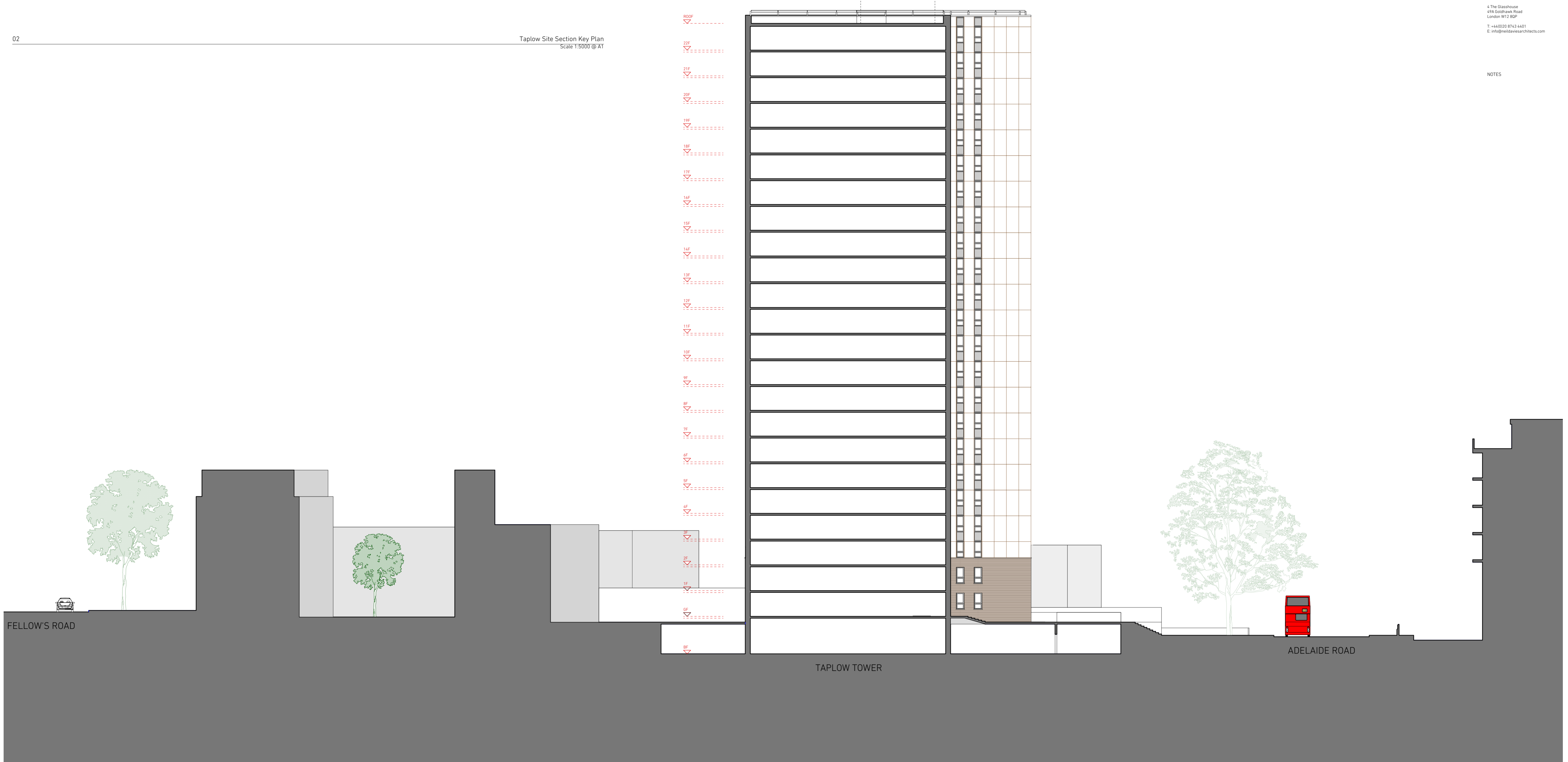
01 Taplow Existing Site Section Scale 1:200 @ A1
