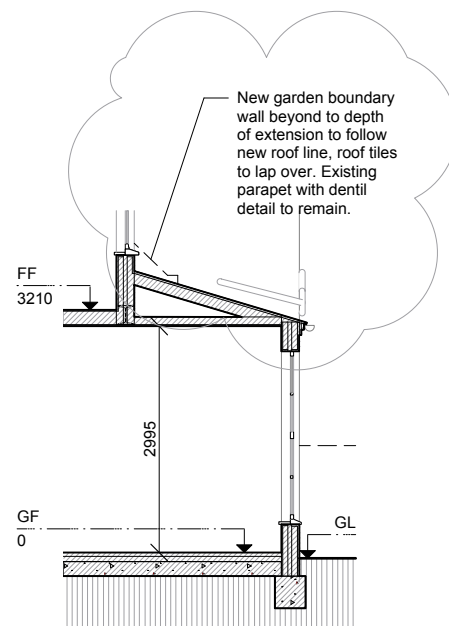
2 Ground floor section - Proposed rear infill 1:100
