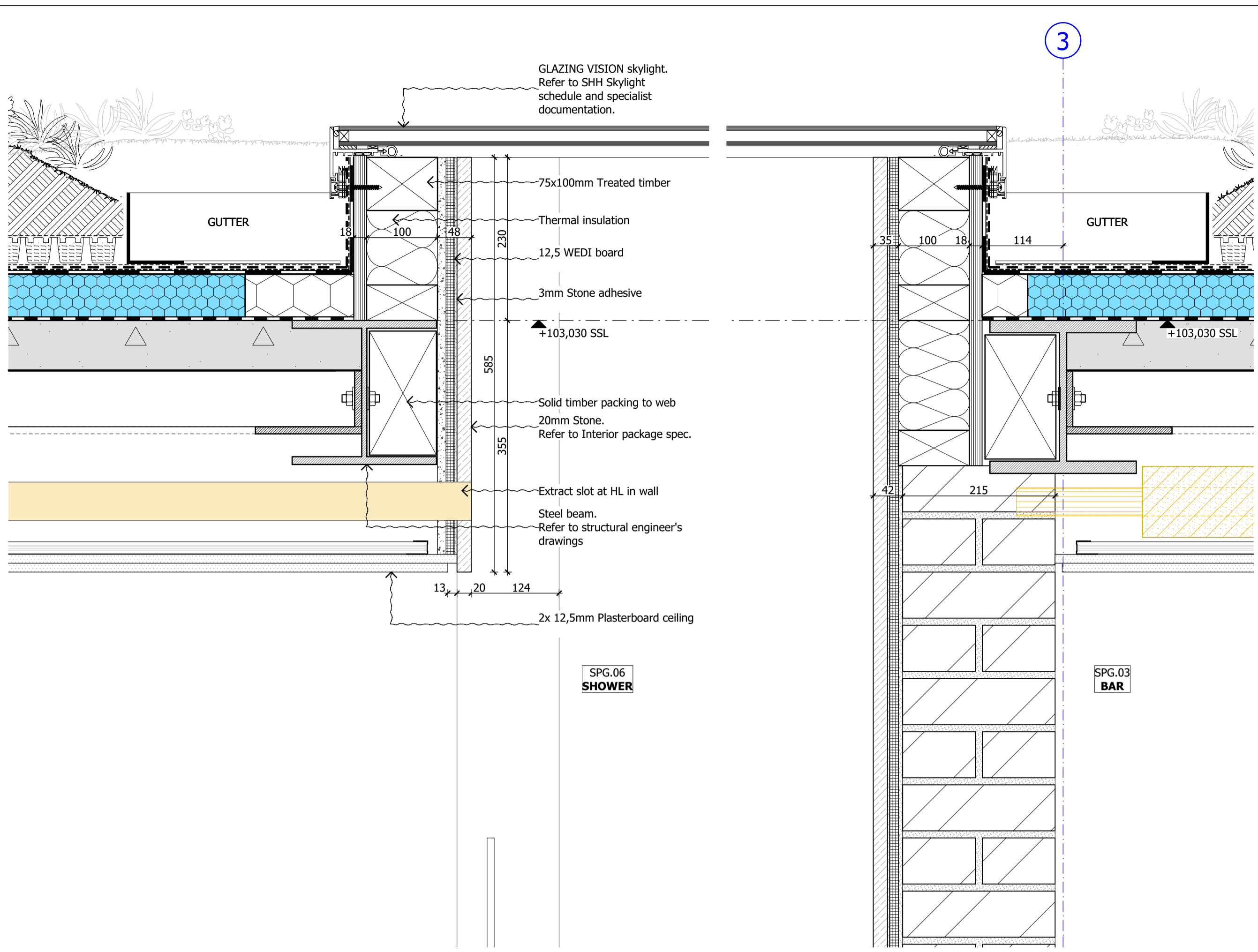
4 SCALE 1:5 @ A1, 1:10 @ A3 ROOF DETAIL THROUGH PROPOSED SKYLIGHT AT SHOWER ROOM- SECTION E
