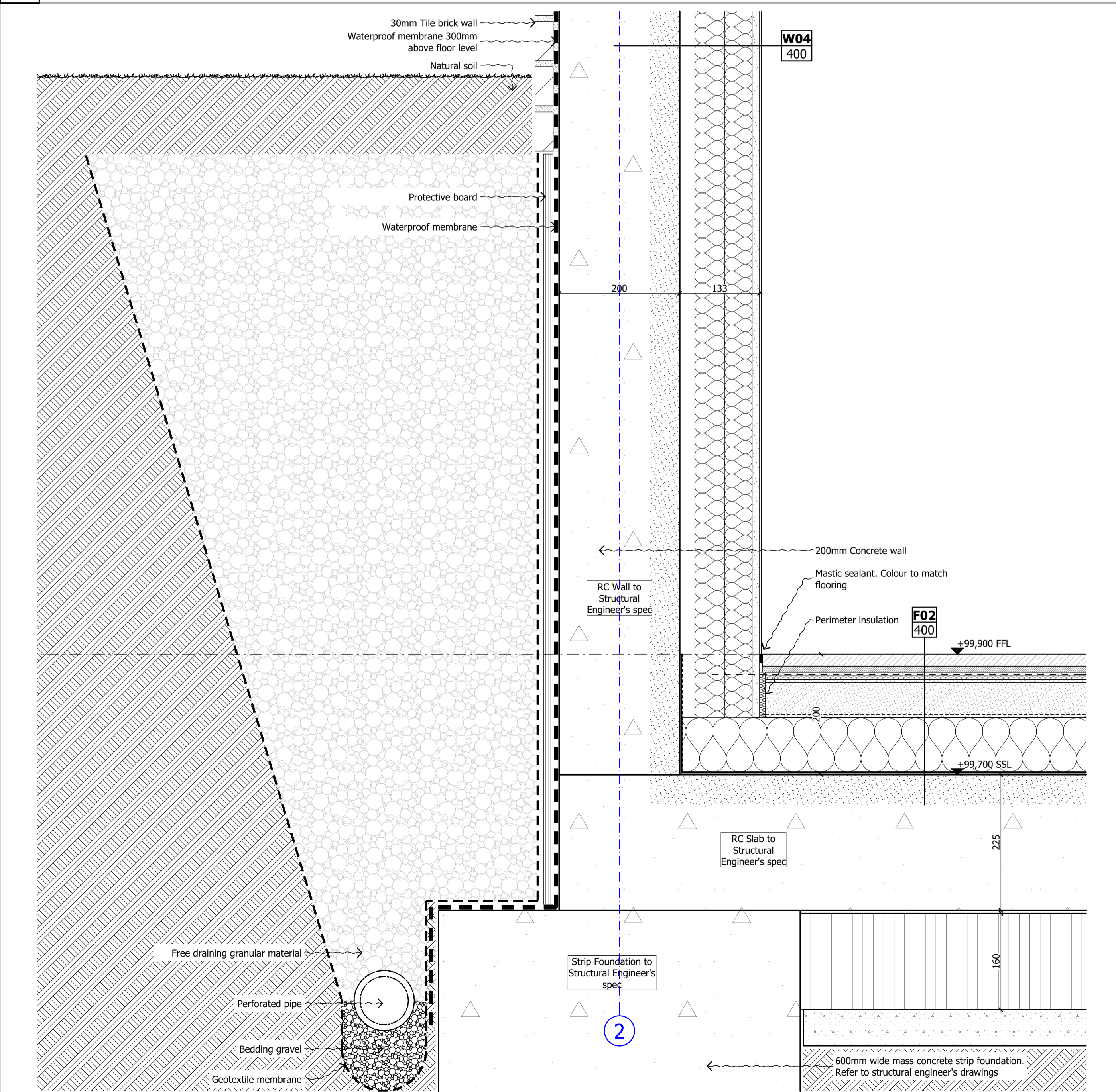
1 SCALE 1:5 @ A1, 1:10 @ A3 FLOOR & WALL DETAIL THROUGH PROPOSED EXTERNAL SOIL - SECTION E
