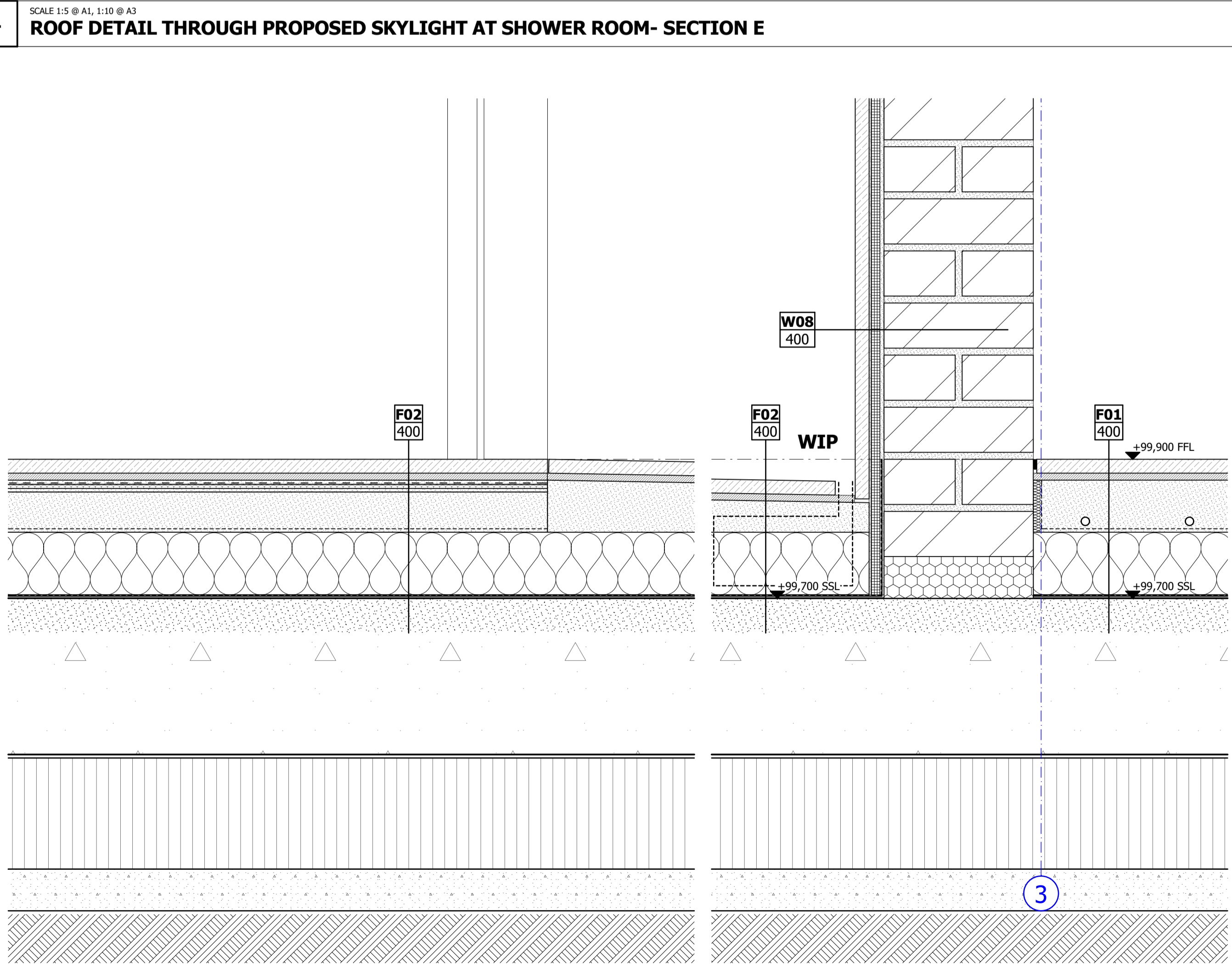
3 SCALE 1:5 @ A1, 1:10 @ A3 FLOOR DETAIL AT SHOWER ROOM- SECTION E
