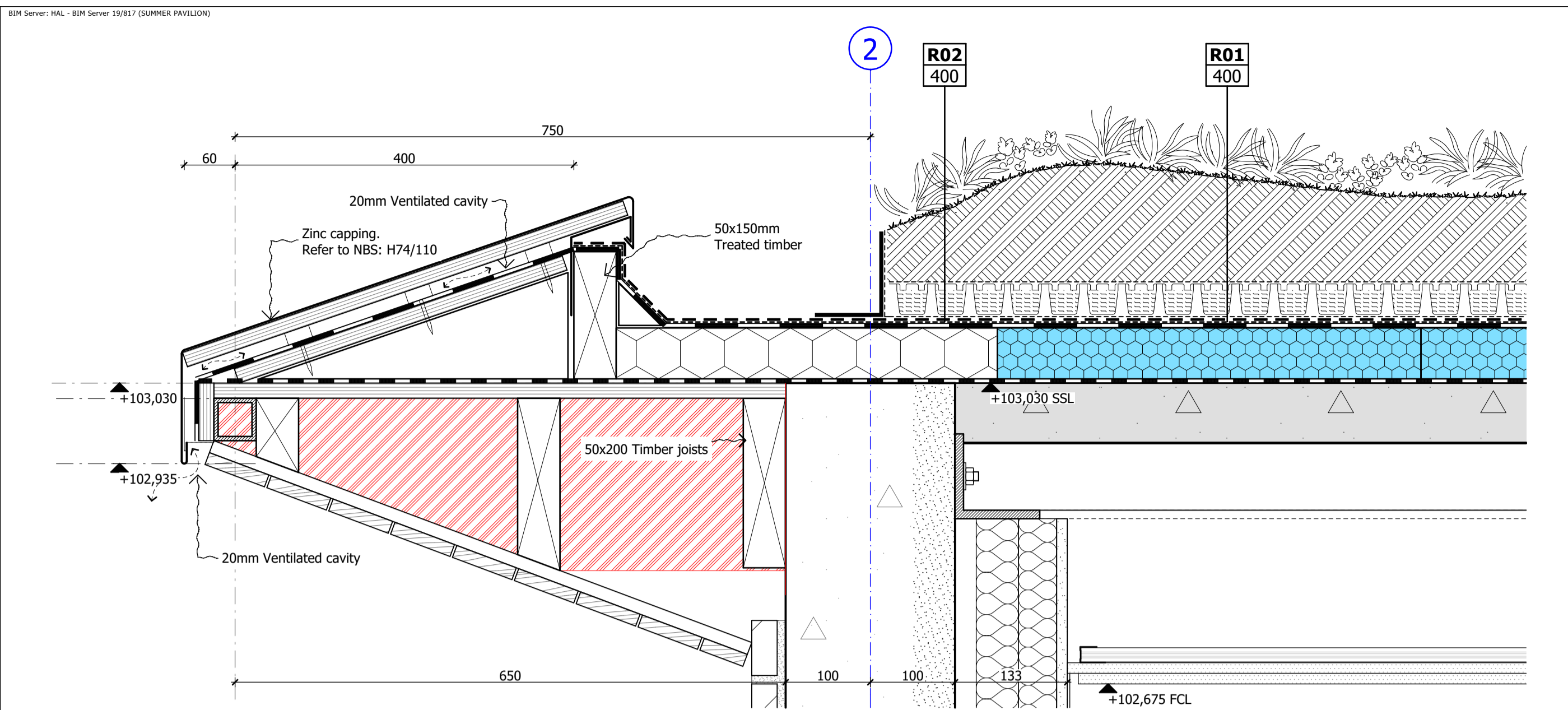
2 SCALE 1:5 @ A1, 1:10 @ A3 ROOF & WALL DETAIL - SECTION E
