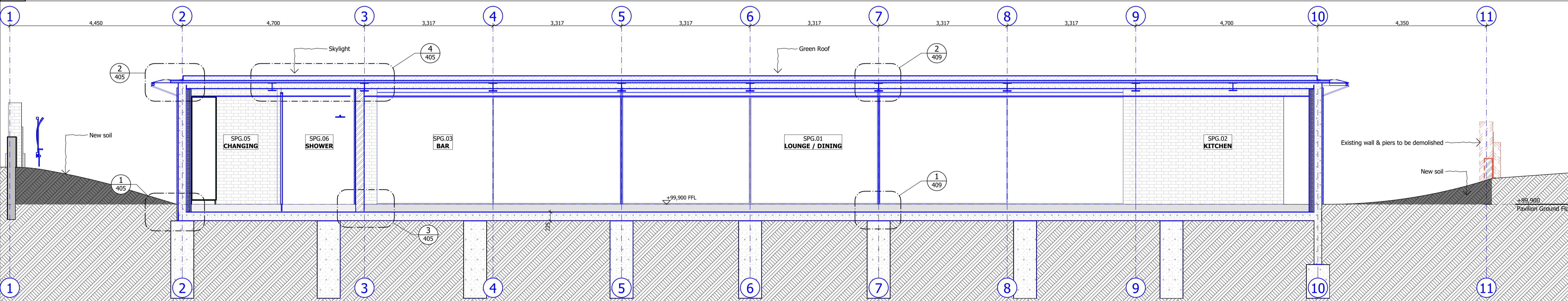
2 SCALE 1:50 @ A0 SUMMER PAVILION - SECTION E
