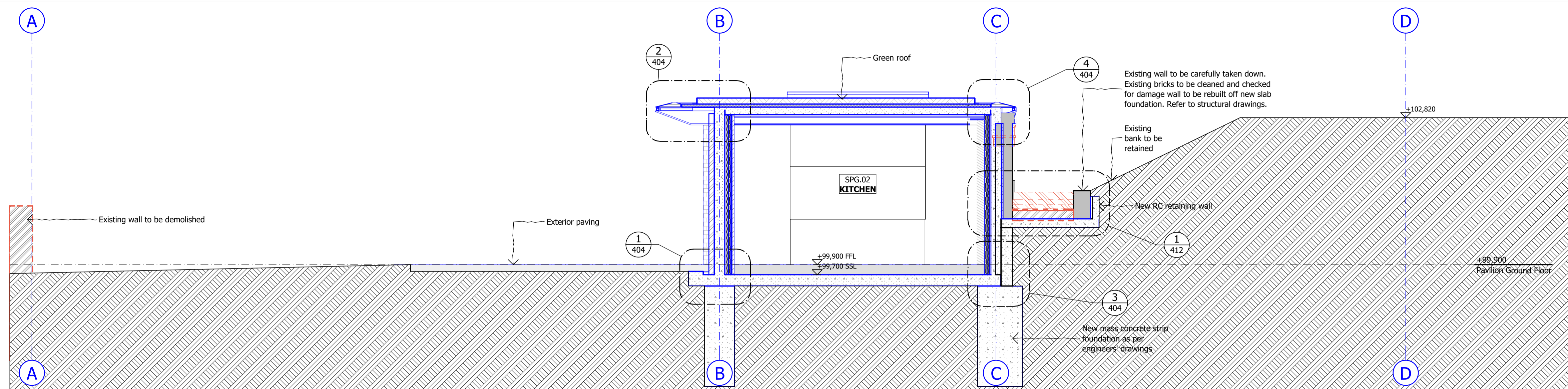
1 SCALE 1:50 @ A1, 1:100 @ A3 SUMMER PAVILION - SECTION D
