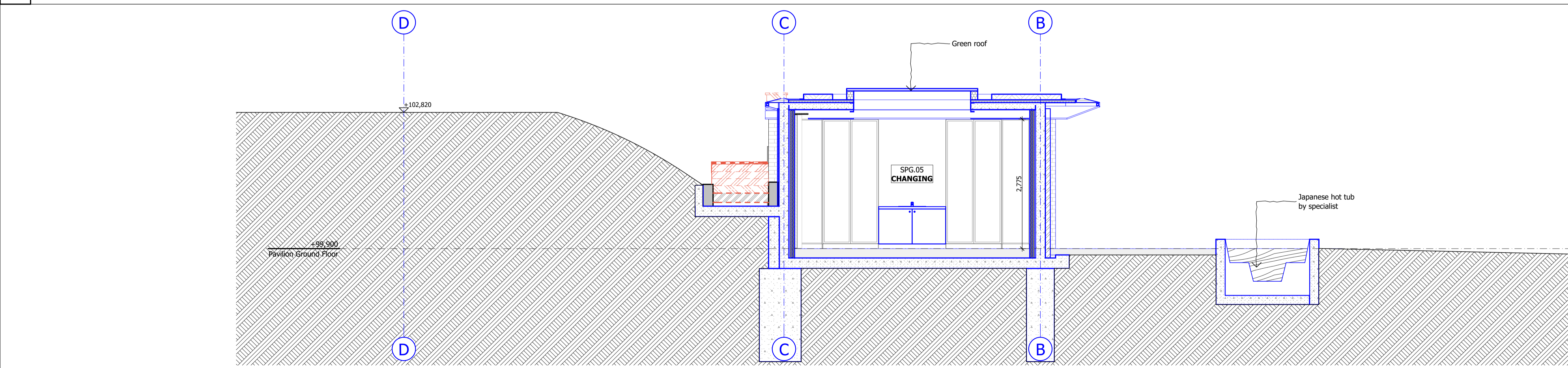
3 SUMMER PAVILION - SECTION C
