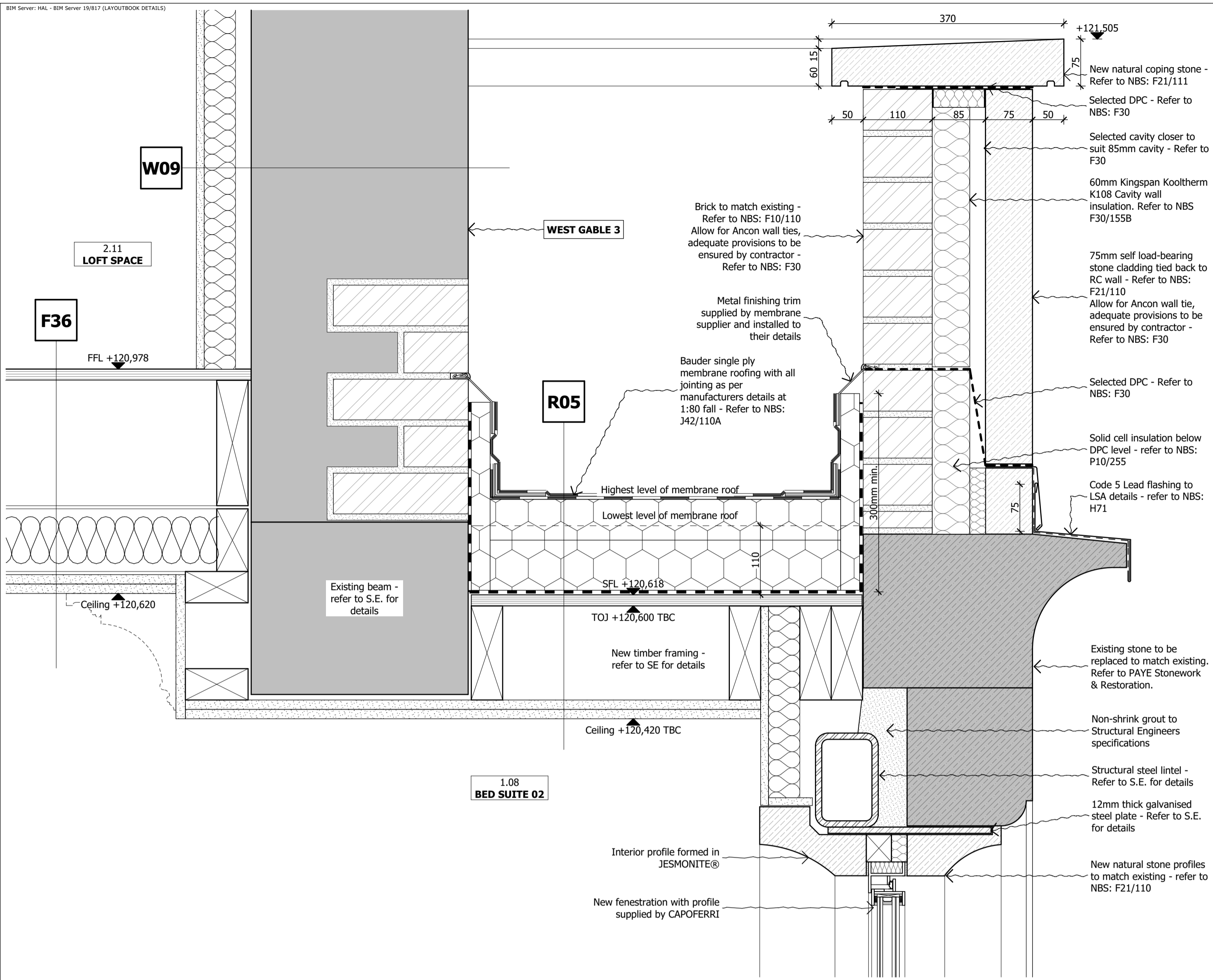
1 SCALE 1:5 @ A1; 1:10 @ A3 SECTION DETAIL - WESTERN SMALL BAY WINDOW WITH PARAPET ROOF
