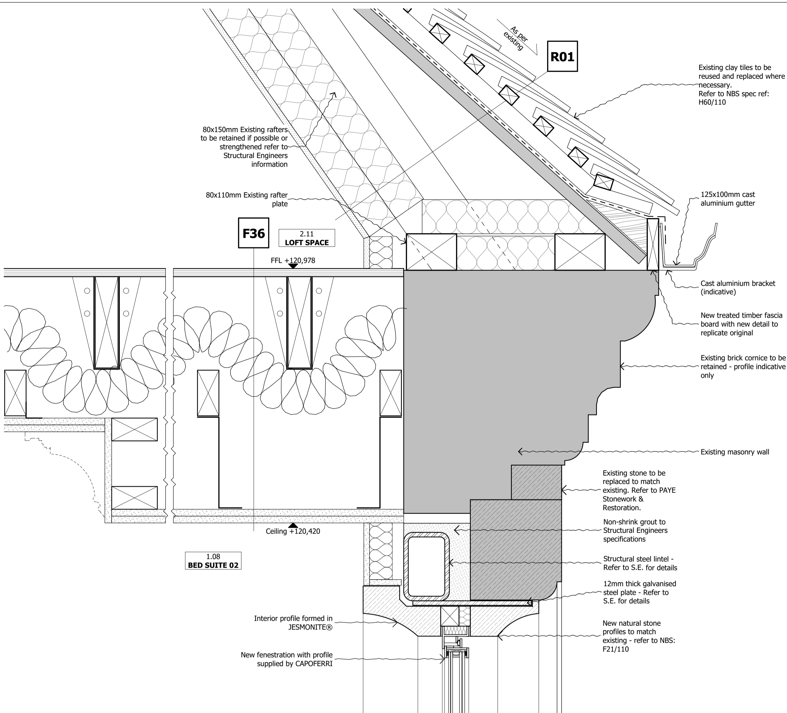
2 SCALE 1:5 @ A1; 1:10 @ A3 SECTION D-D DETAIL - SOUTHERN SMALL BAY WINDOW WITH PITCHED TILED ROOF
