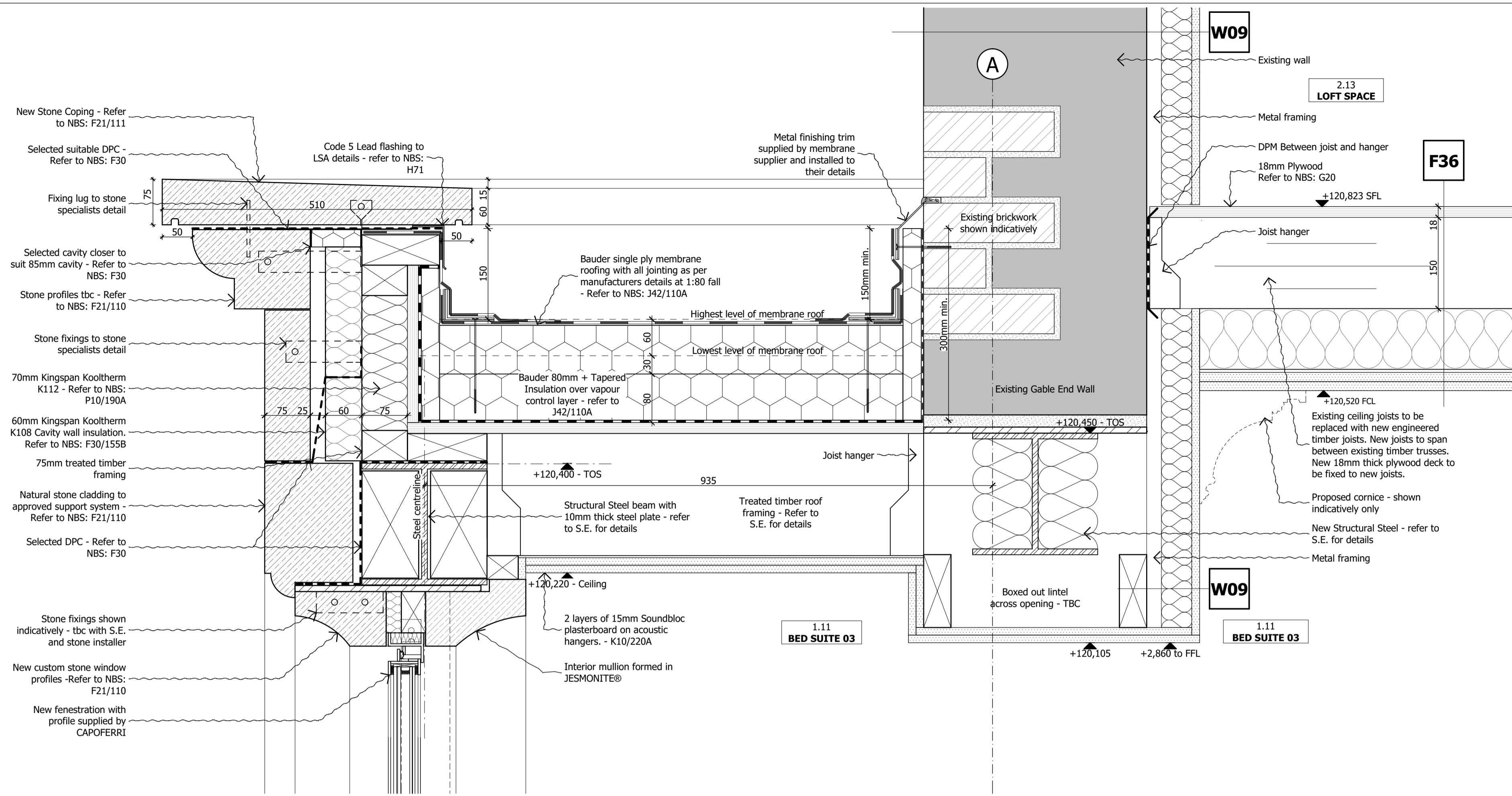
1 SCALE 1:5 @ A1; 1:10 @ A3 MEMBRANE ROOF TO NEW BAY WINDOW TO BEDROOM 03 DETAIL
