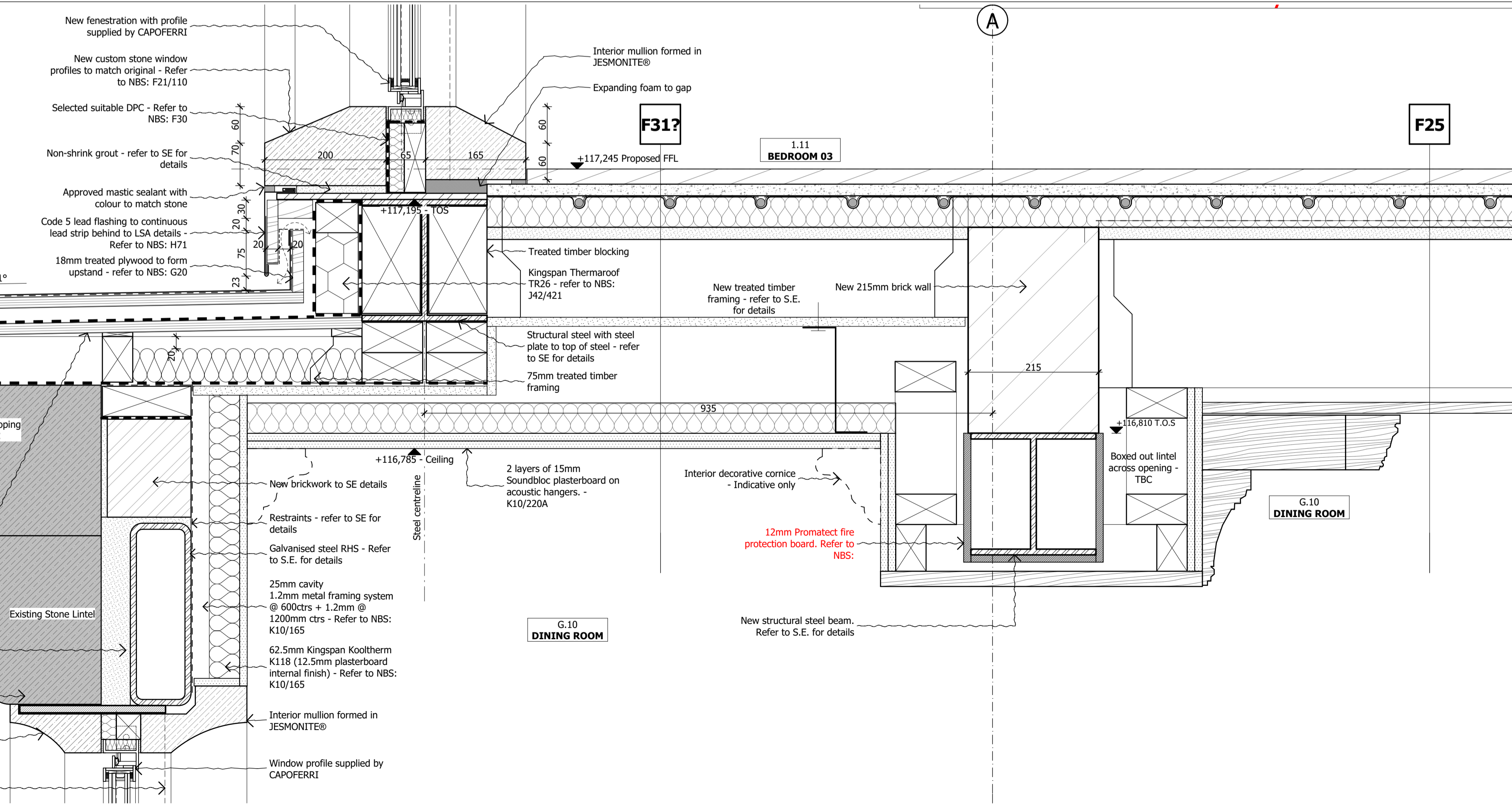
2 SCALE 1:5 @ A1; 1:10 @ A3 NEW BAY WINDOW SILL TO EXSITING BAY WINDOW HEAD SECTION DETAIL
