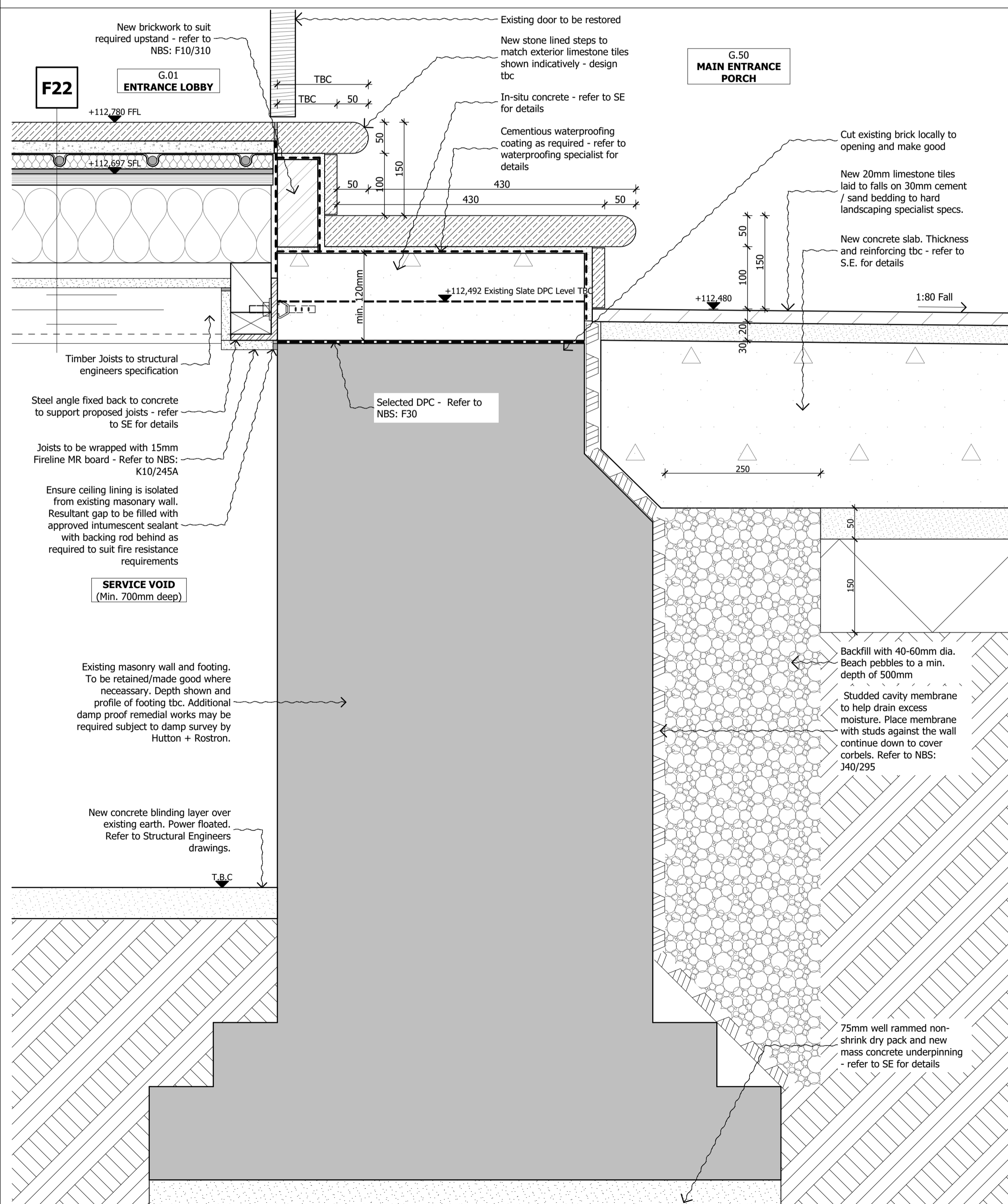
1 SCALE 1:5 @ A1; 1:10 @ A3 SECTION B-B DETAIL - GROUND FLOOR MAIN DOOR THRESHOLD IN EXISTING WALL
