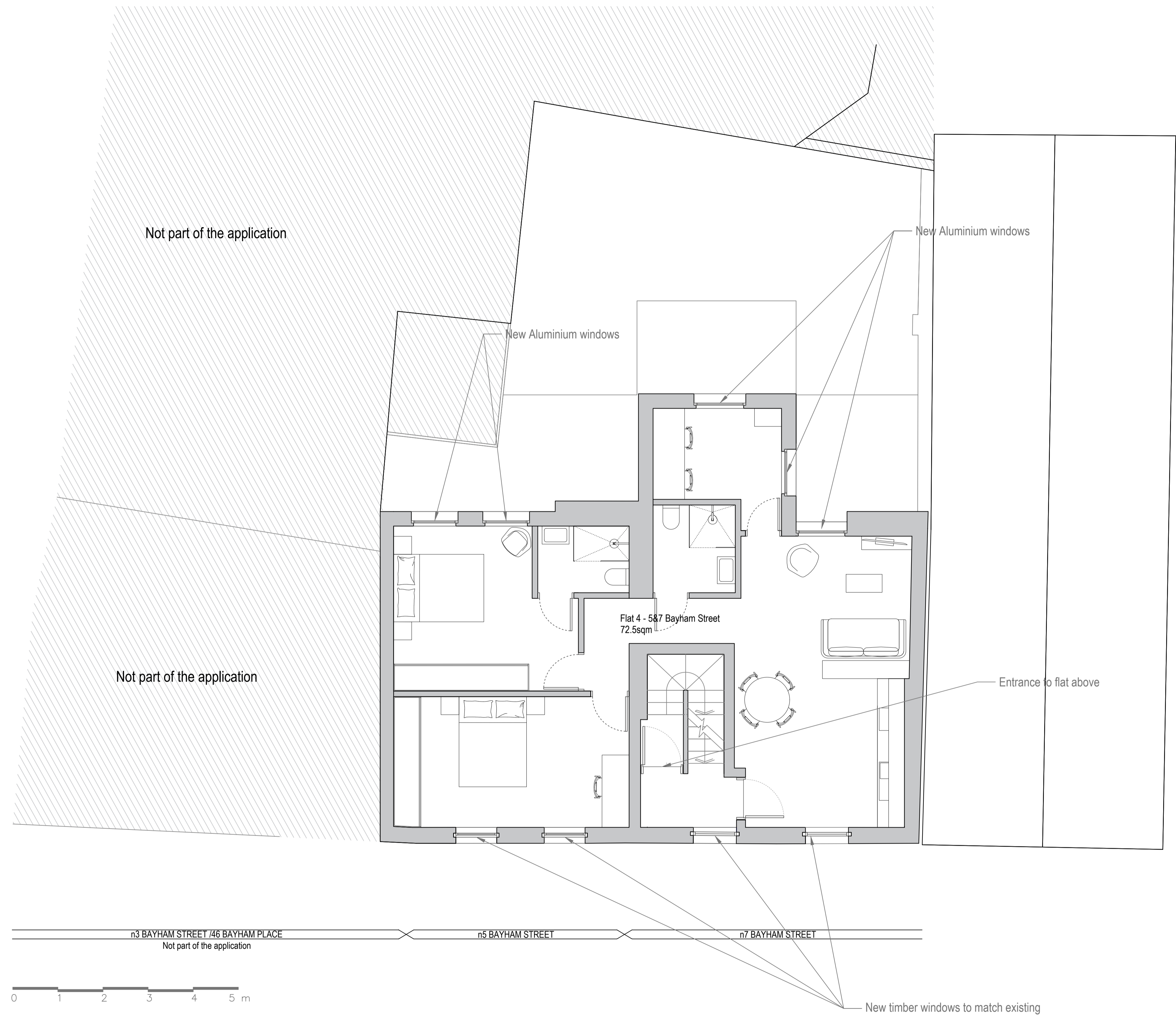
SECOND FLOOR PLAN PR-0103
