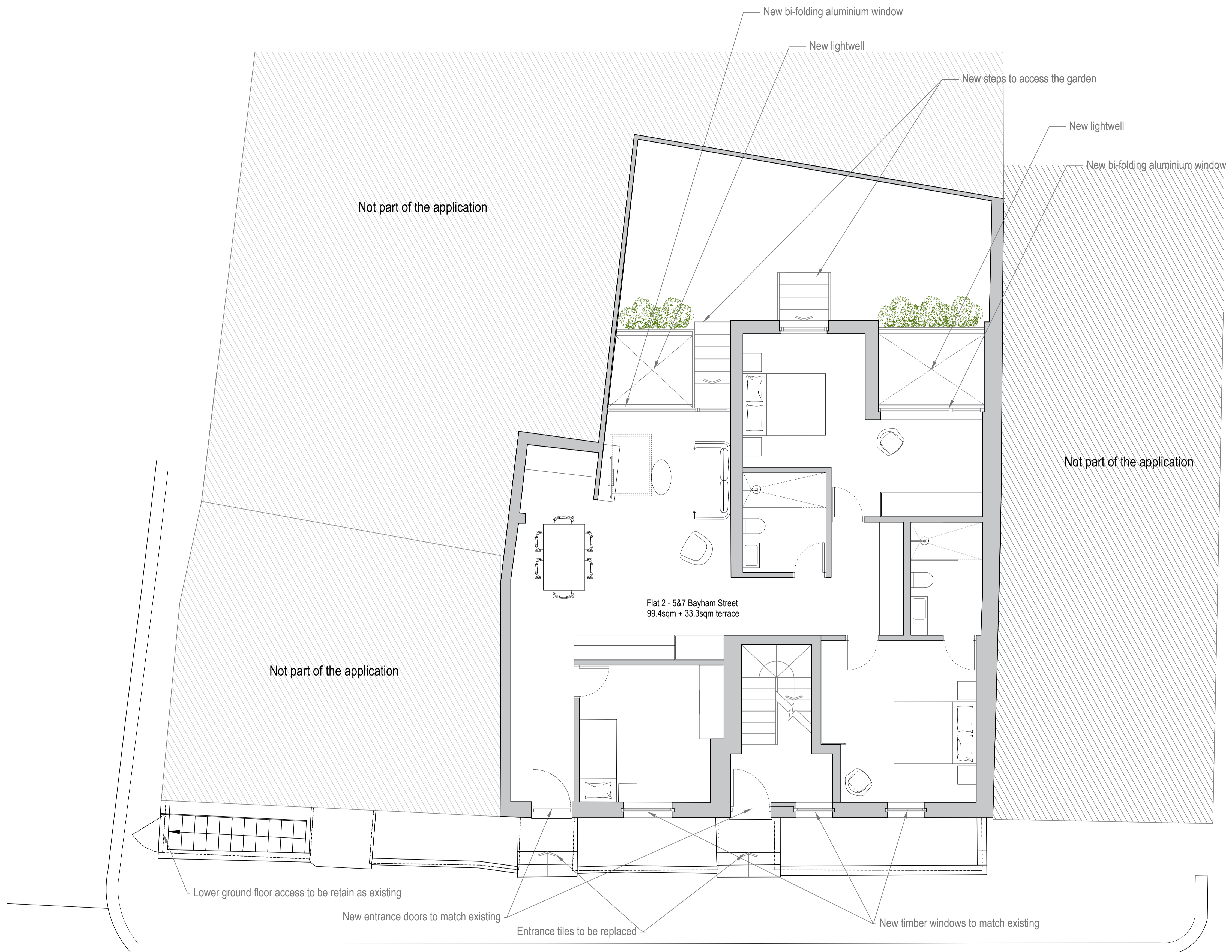
GROUND FLOOR PLAN PR-0101
