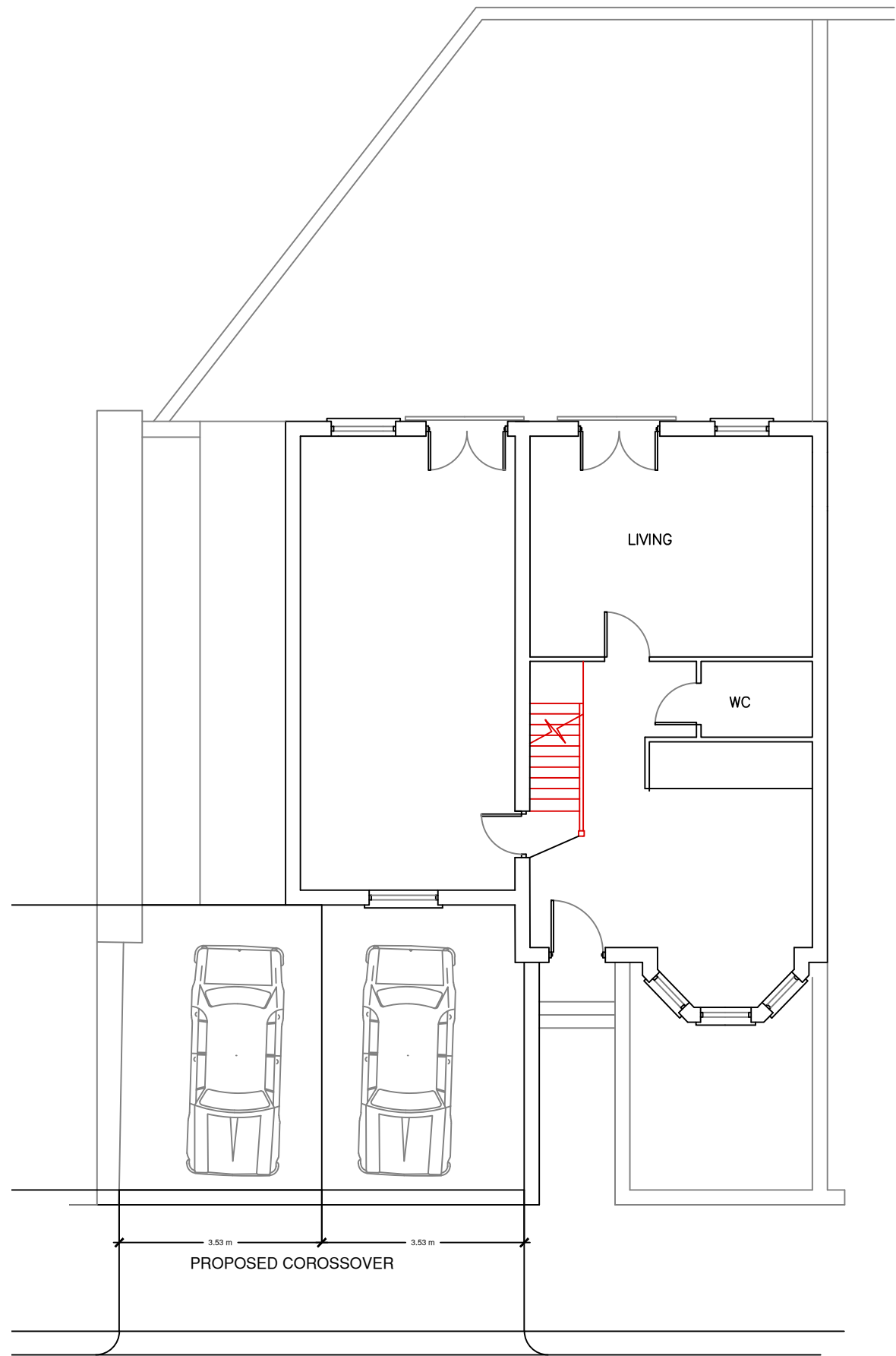
GROUND FLOOR PLAN SHOWING NEW FRONT CAR PARKING SPACES
