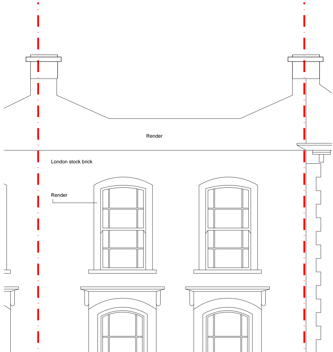
Existing Front Elevation 1:50 @ A3
