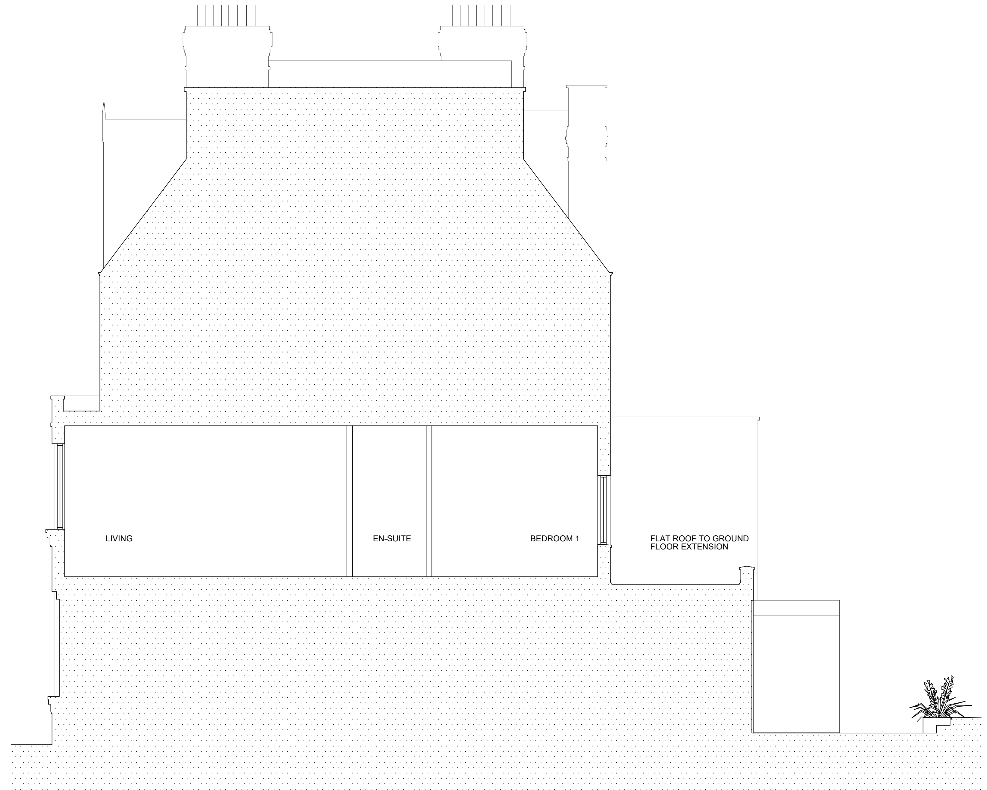
Existing Section 1:100 Showing Approved Extension Planning Ref. 2105/5097/P
