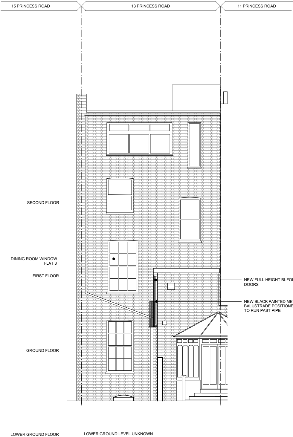
1 PROPOSED REAR ELEVATION 1:100
