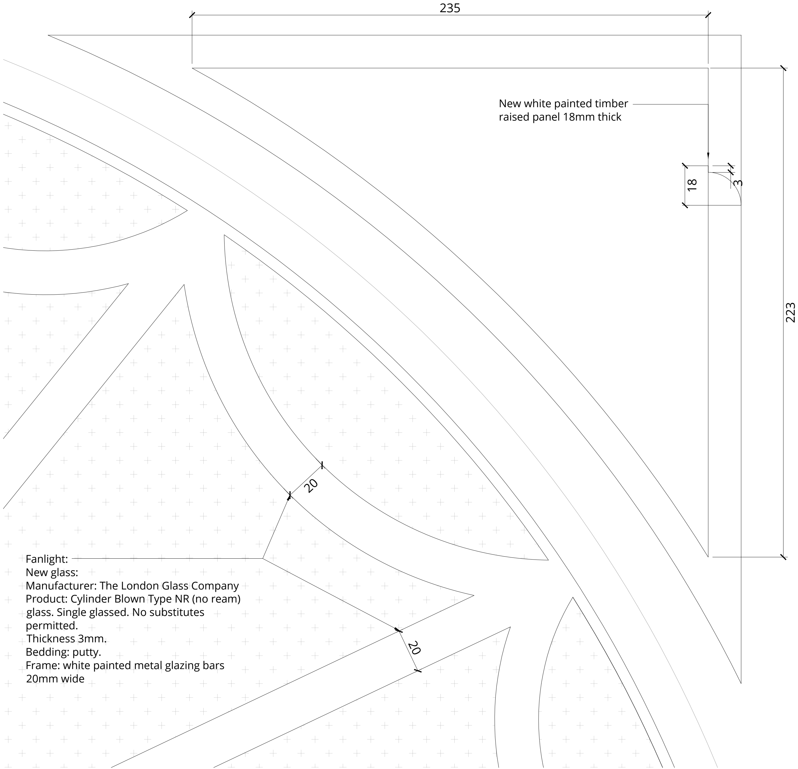
02 PROPOSED ELEVATION DETAIL FANLIGHT 1:1@A1
