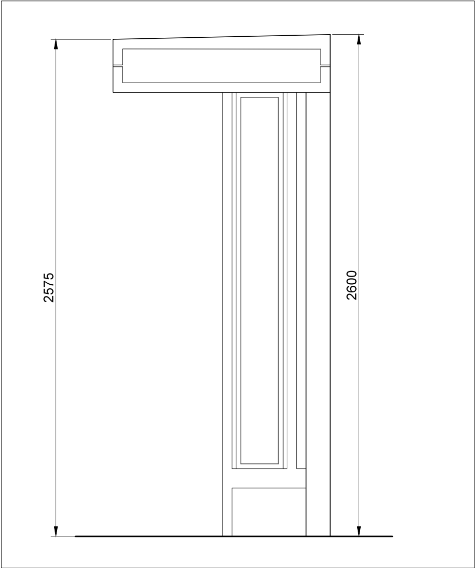
04 Side Elevation
