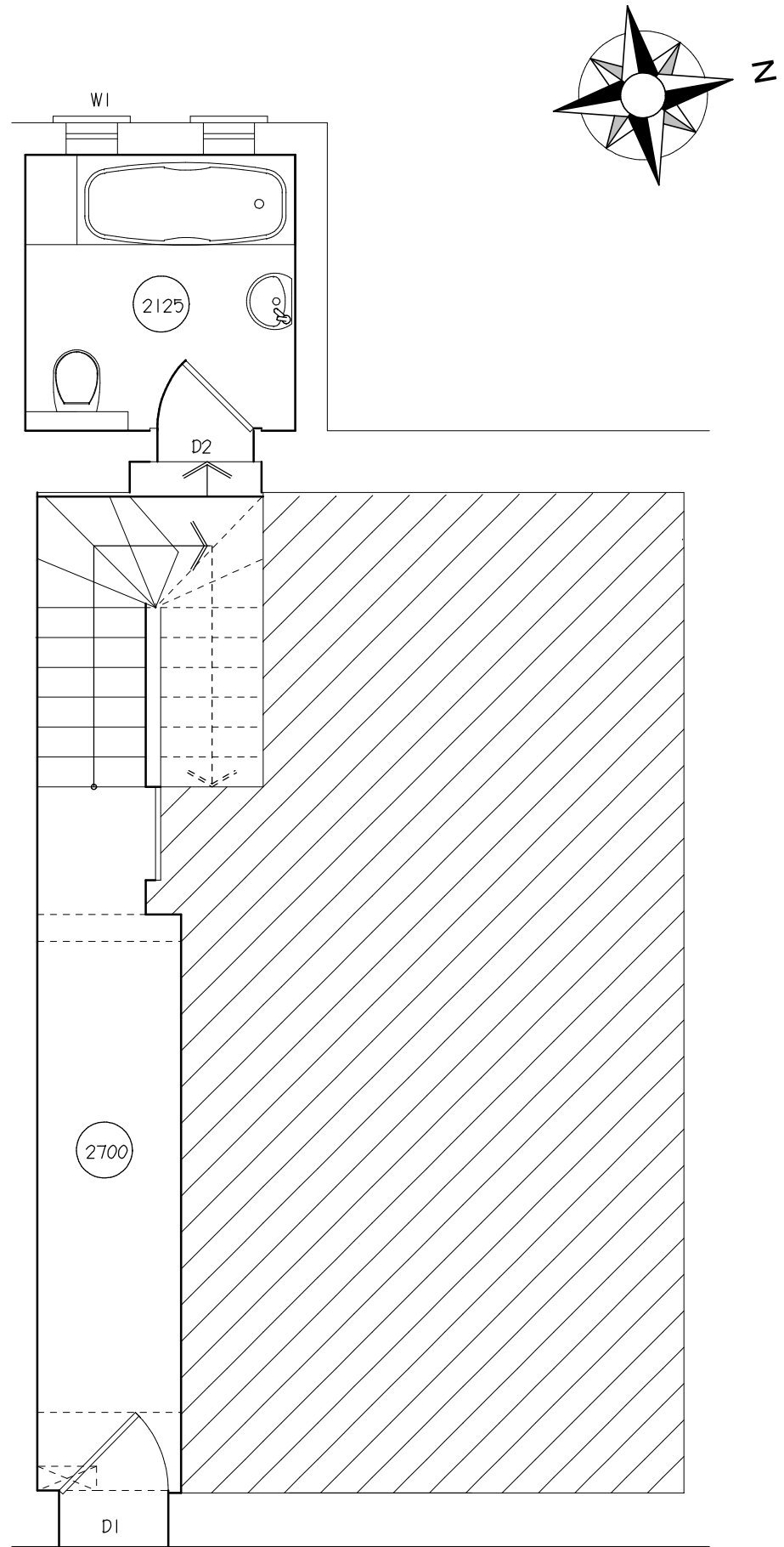
↑ CONDITION SURVEY - GROUND FLOOR PLAN - entrance level
