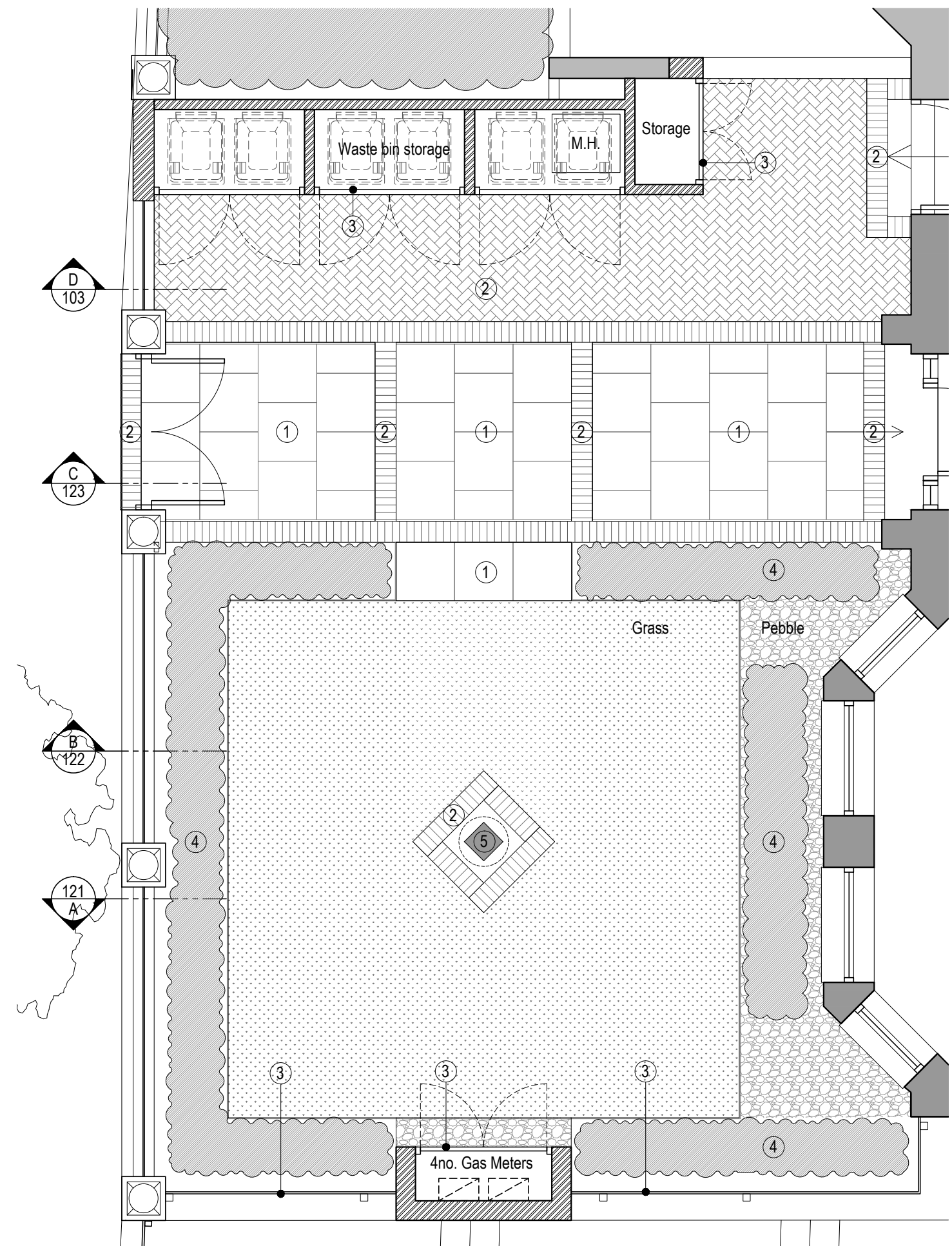
Proposed Front Garden Plan Scale 1:50 @ A3
