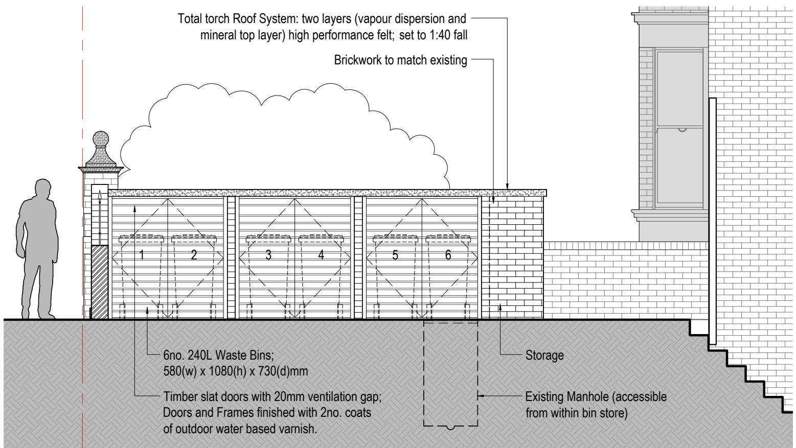
Proposed Bin Store Elevation (D) Scale 1:50 @ A3
