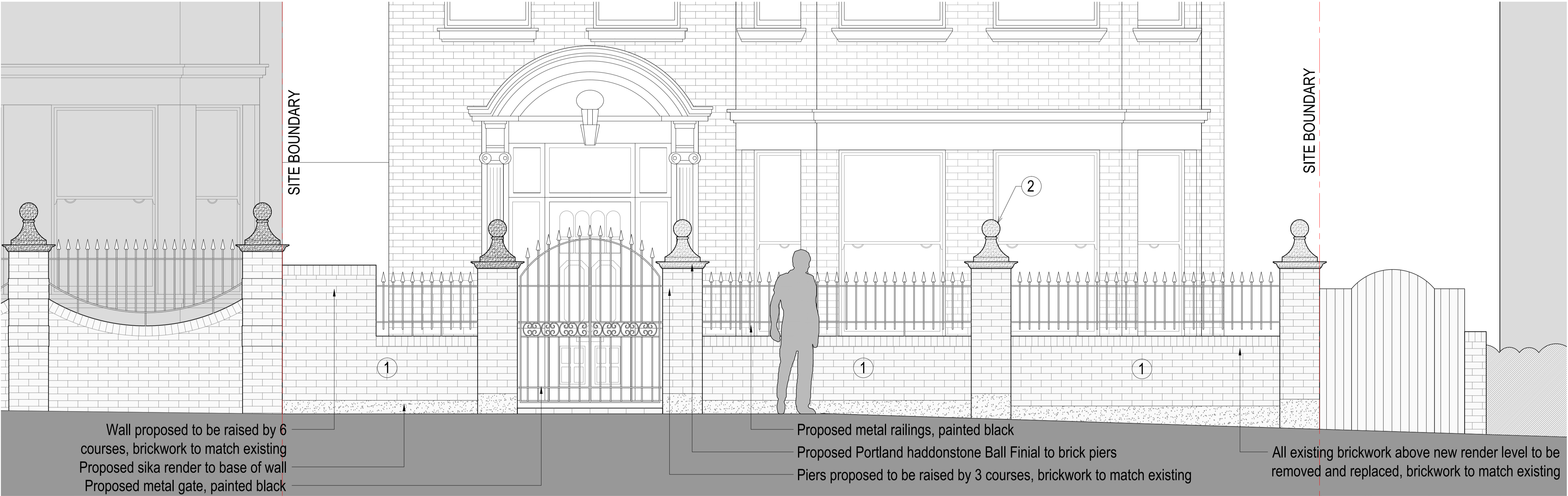
Proposed Street Elevation Scale 1:50 @ A3
