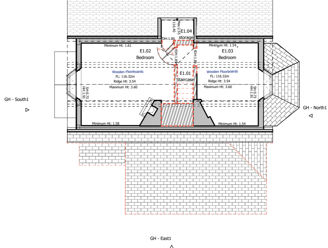
2 GATE HOUSE - FIRST FLOOR GA - DEMOLITION
