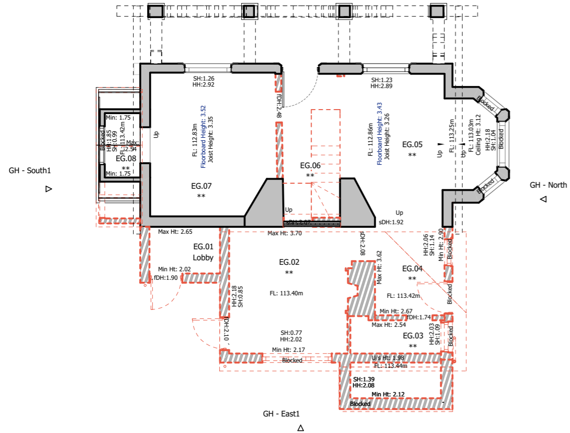
1 GATE HOUSE - GROUND FLOOR GA - DEMOLITION
