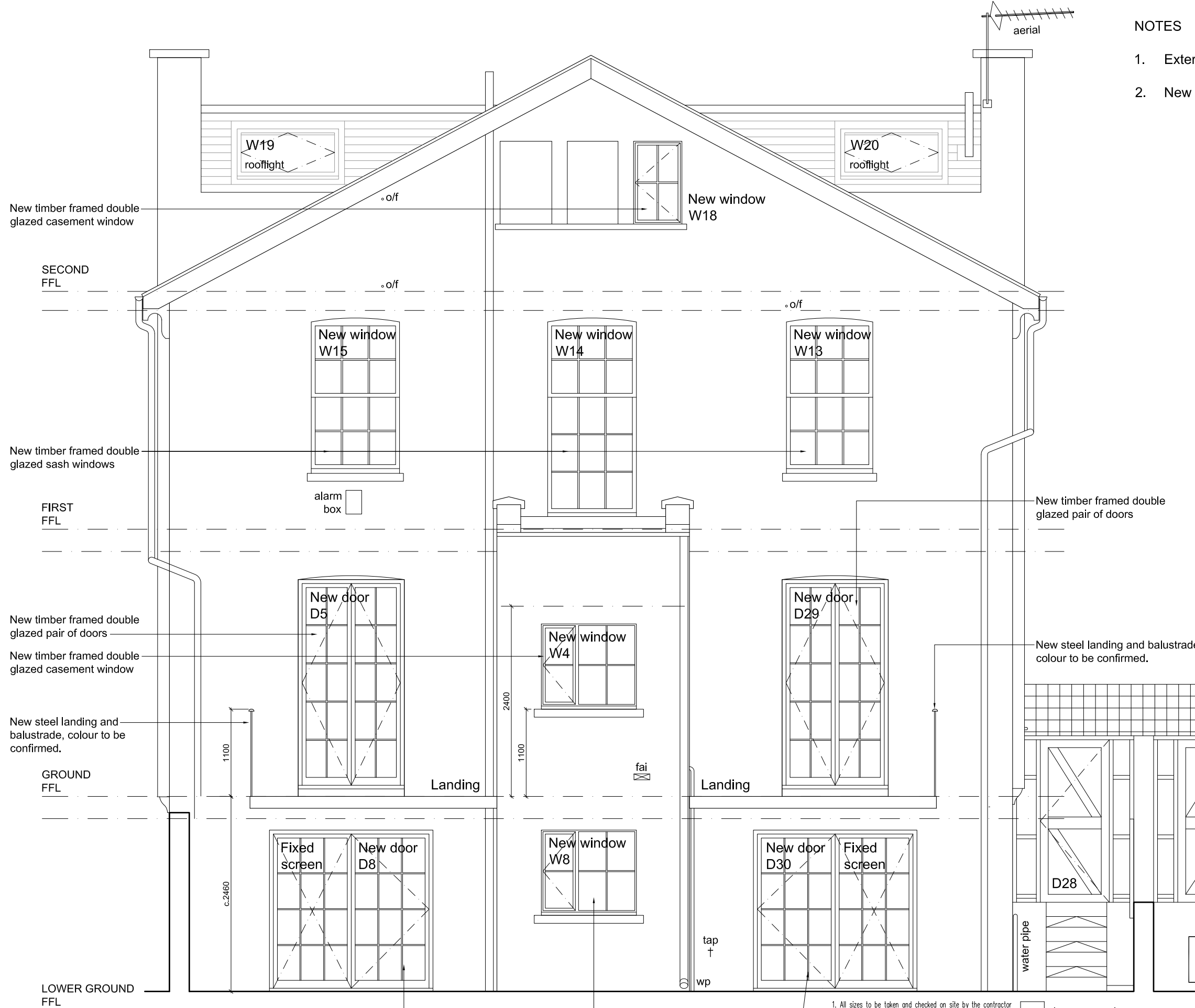
Rear Elevation as Proposed (view on landing) Scale 1:50 @ A3
