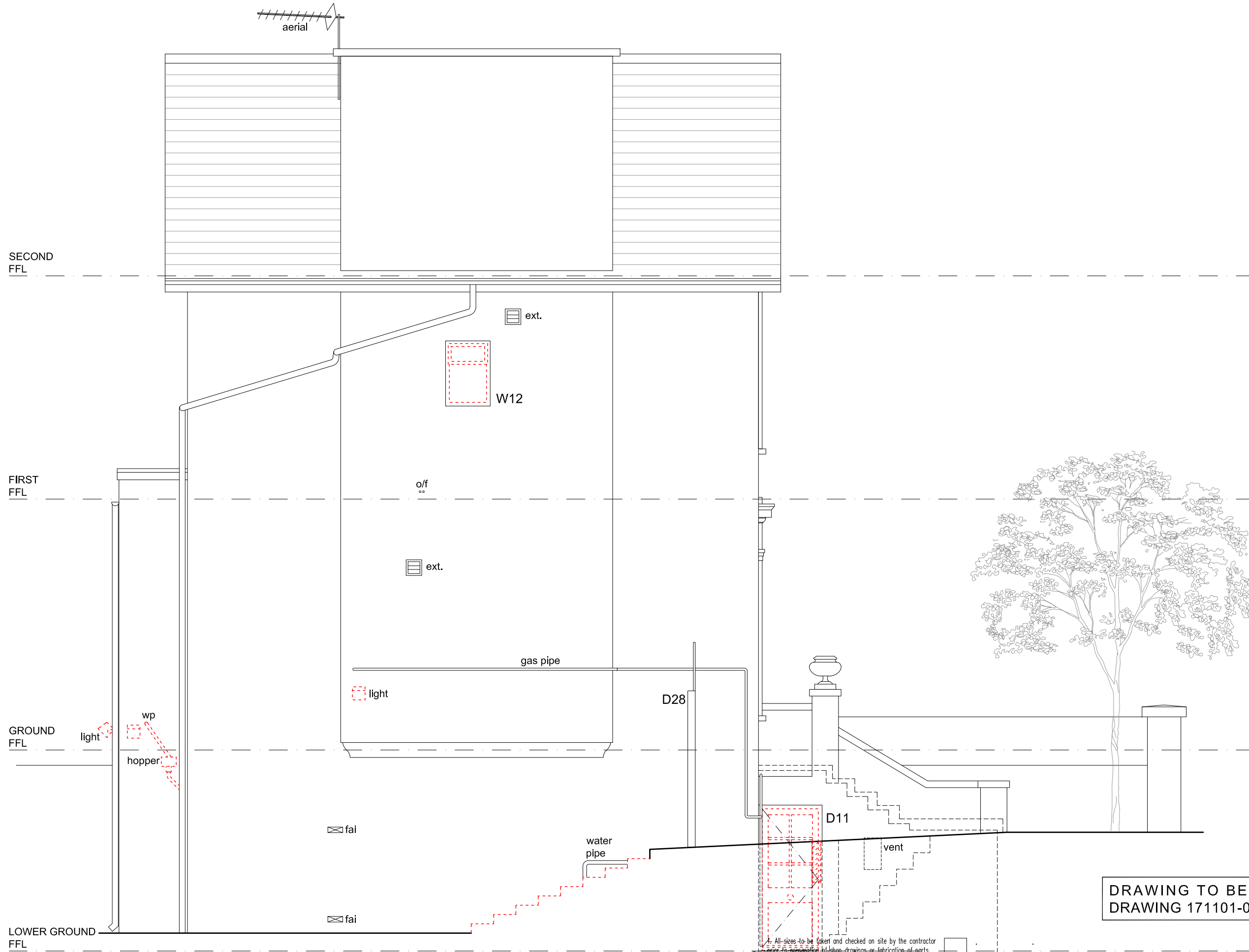
Side Elevation 1 as Existing Scale 1:50 @ A3
