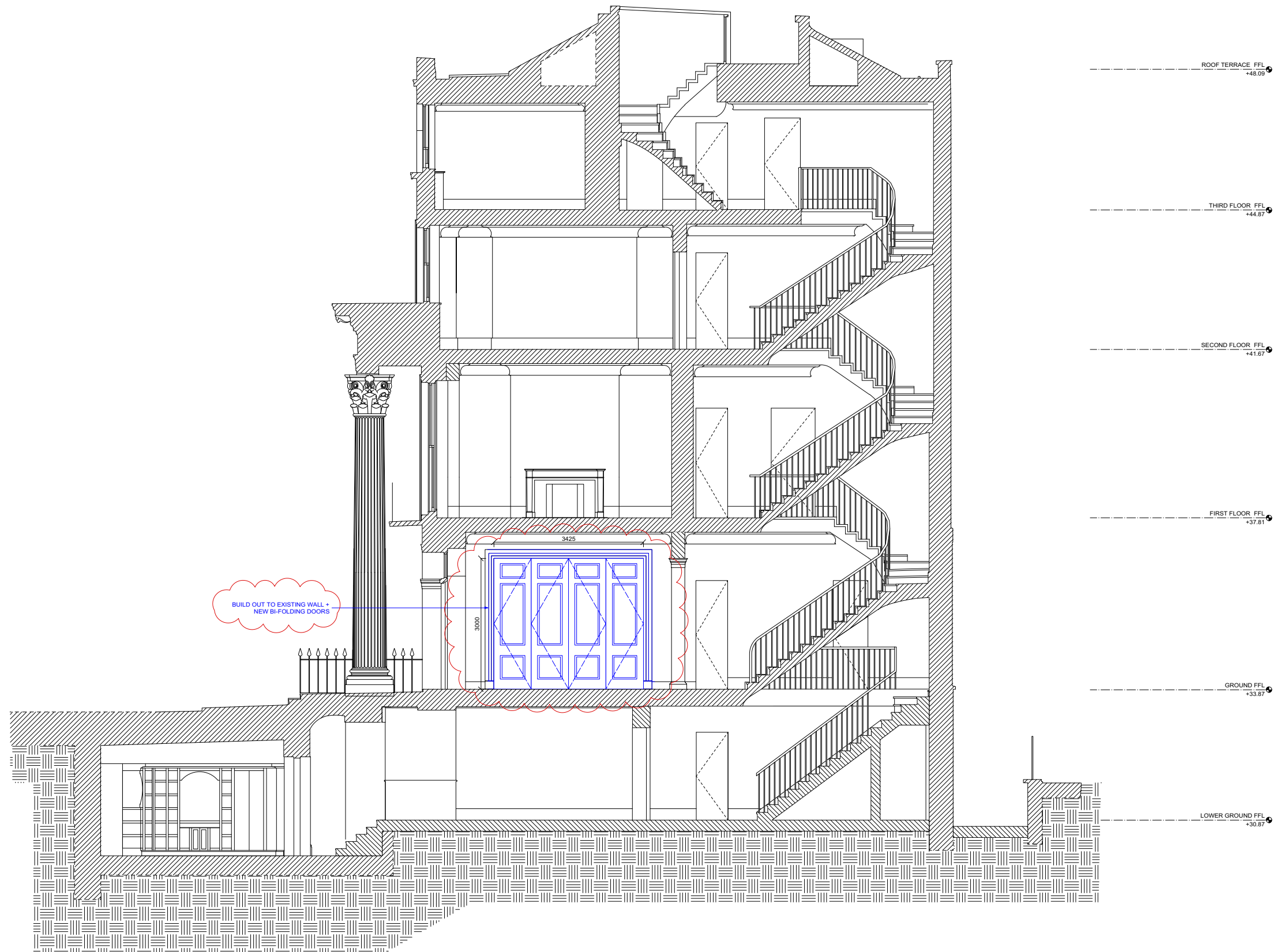
1 PROPOSED SECTION A-A SCALE 1:50
