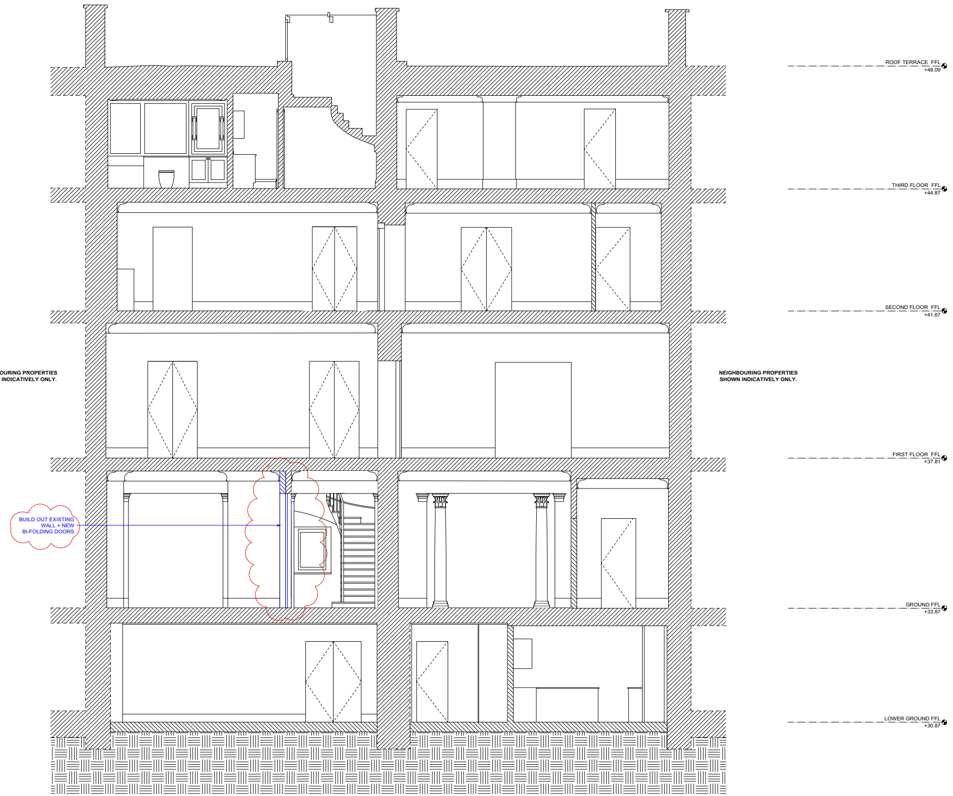
1 PROPOSED SECTION B-B PL-24 SCALE 1:50
