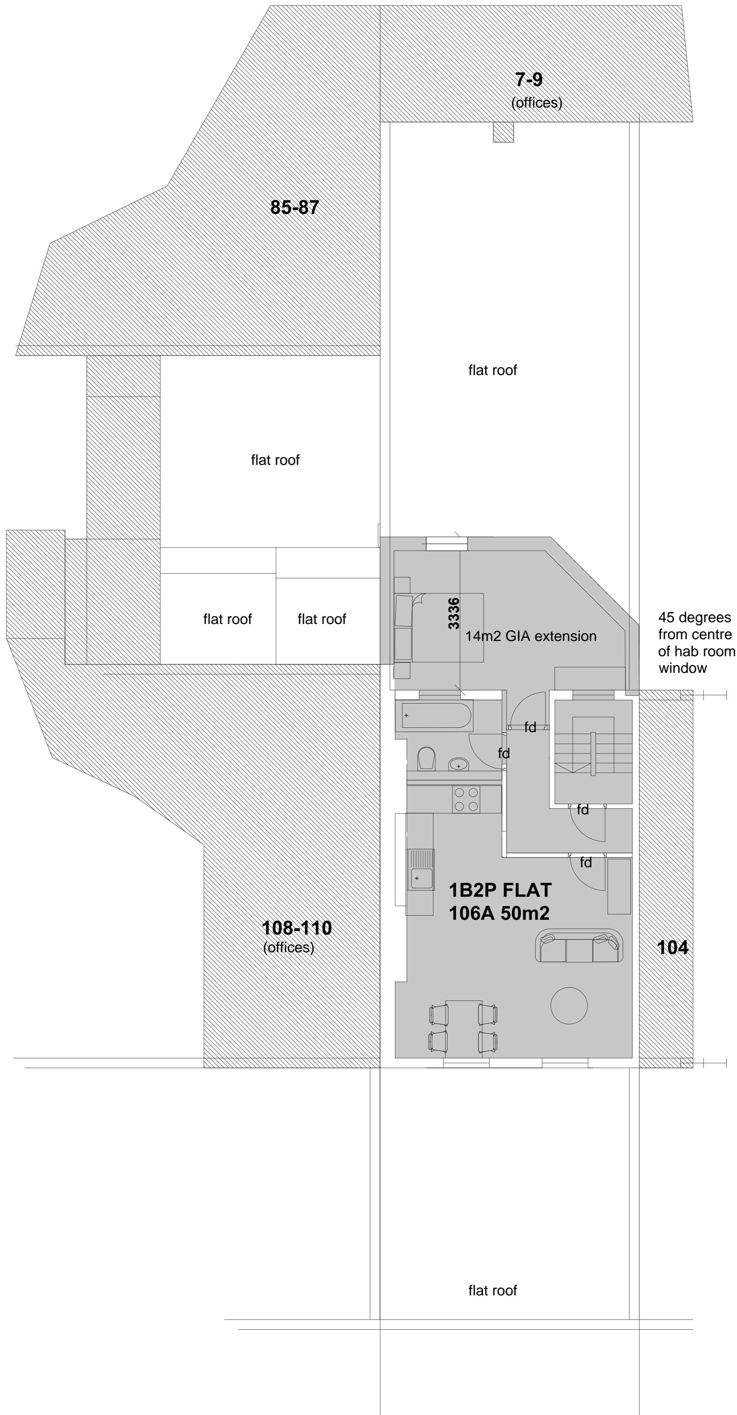
FIRST FLOOR PLAN
