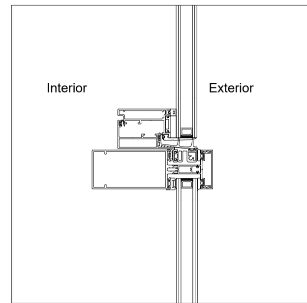
TRANSOM (OPENABLE/FIXED)
