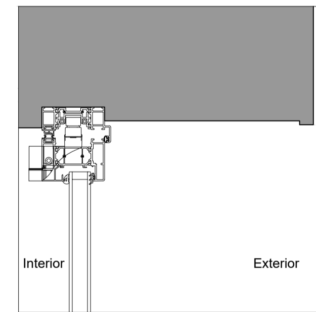
HEAD
