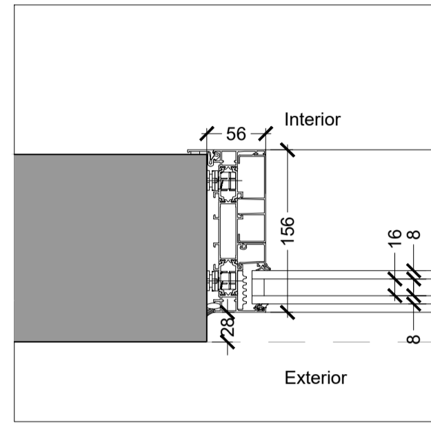
JAMB (FIXED)
