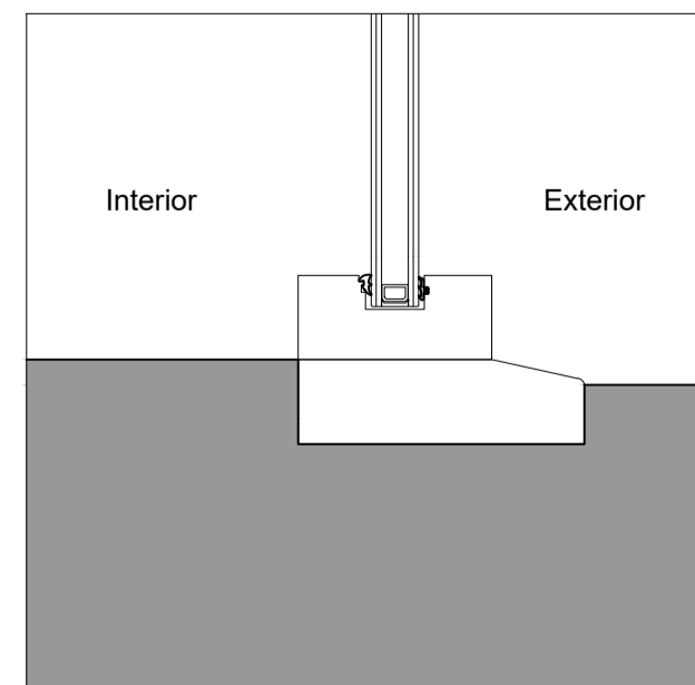
SILL (SIDELIGHT)
