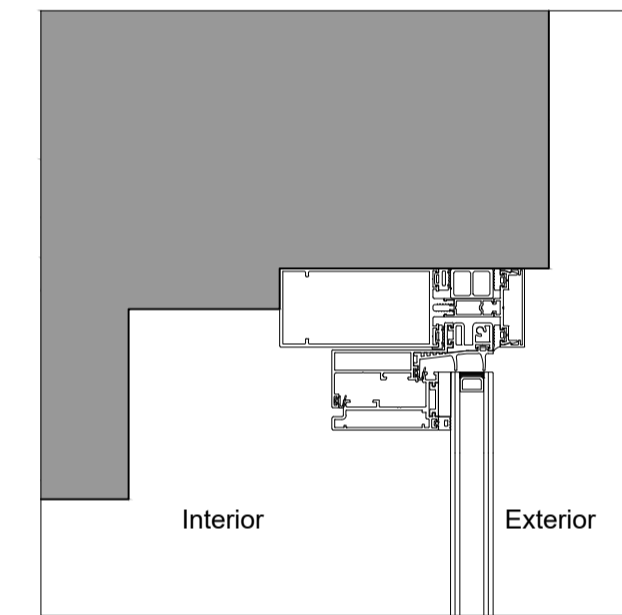
HEAD (OPENABLE)
