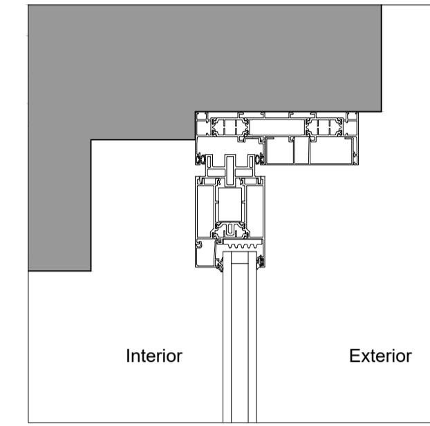
HEAD (DOOR)
