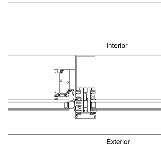
MULLION (OPENABLE/FIXED)
