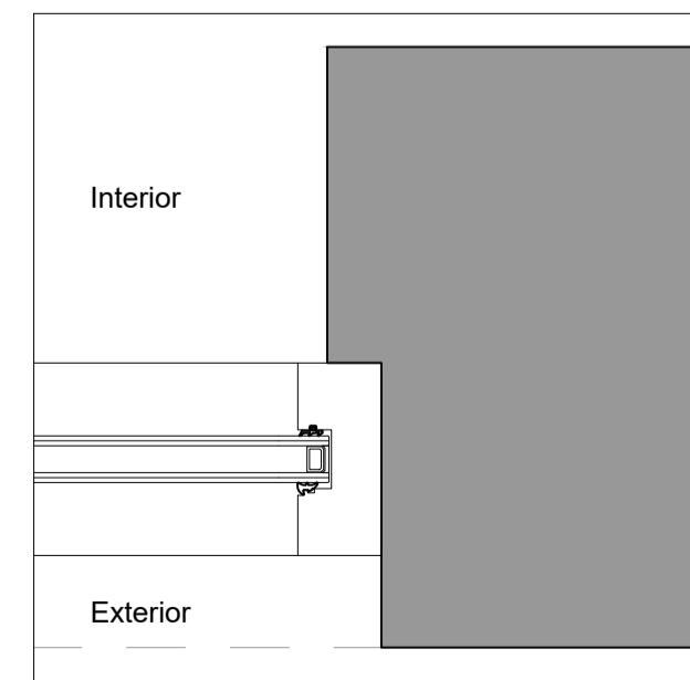
JAMB (SIDELIGHT)
