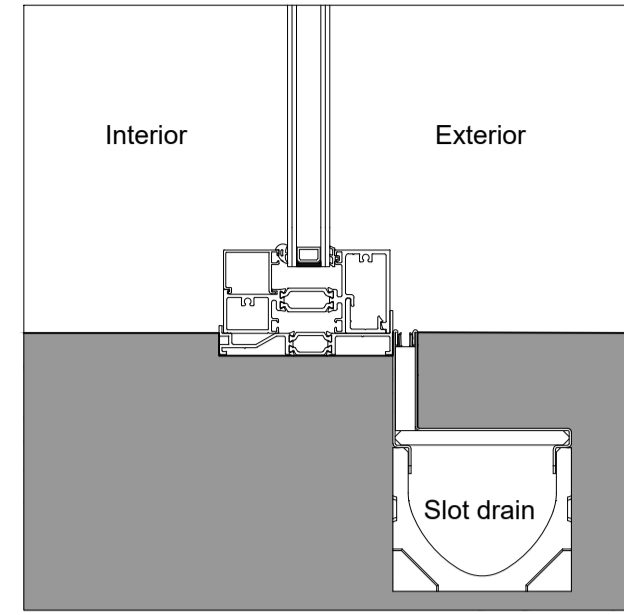
SILL (SIDE LIGHT)
