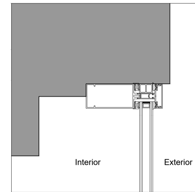
HEAD (FIXED)
