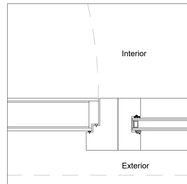
MULLION (DOOR/SIDELIGHT)
