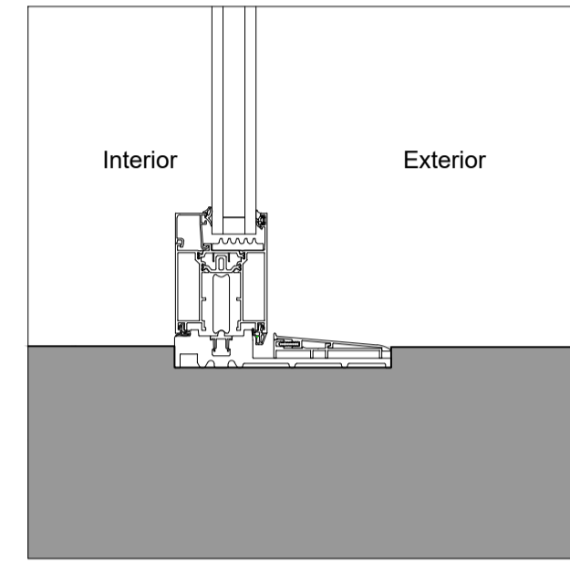
SILL (DOOR)
