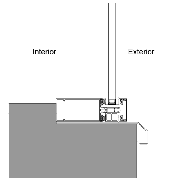
SILL
