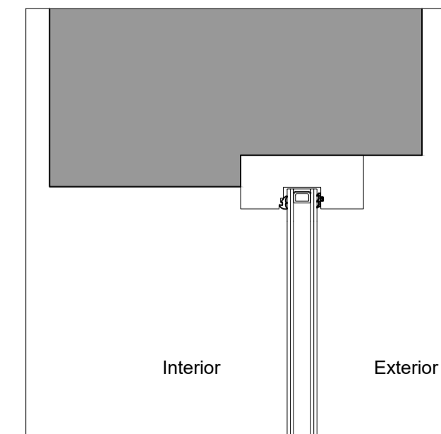
HEAD (SIDELIGHT)
