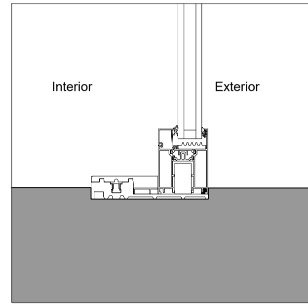
SILL (FIXED)
