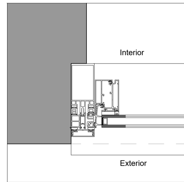
JAMB (OPENABLE)
