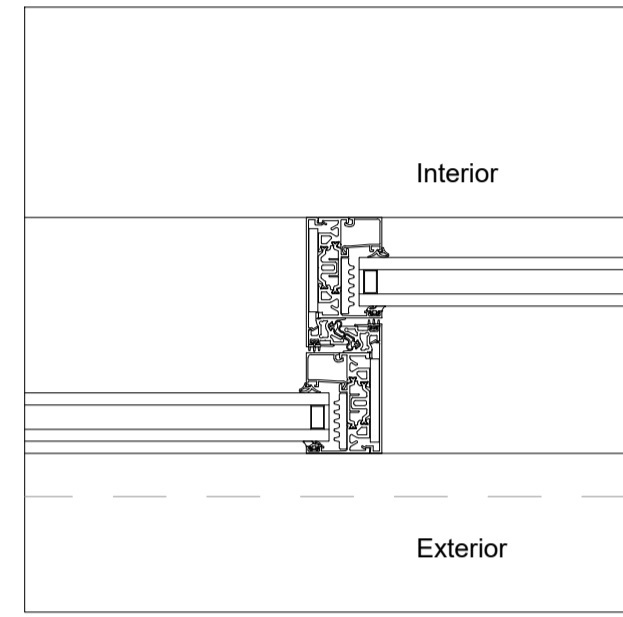
MULLION (FIXED/DOOR)
