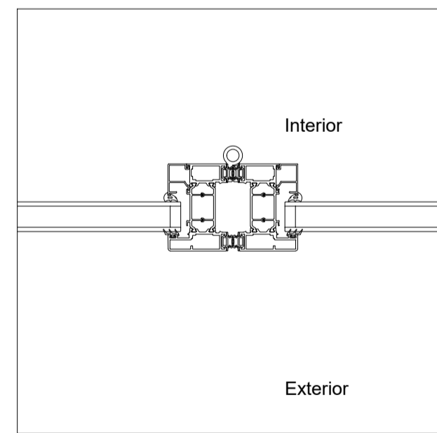
MULLION
