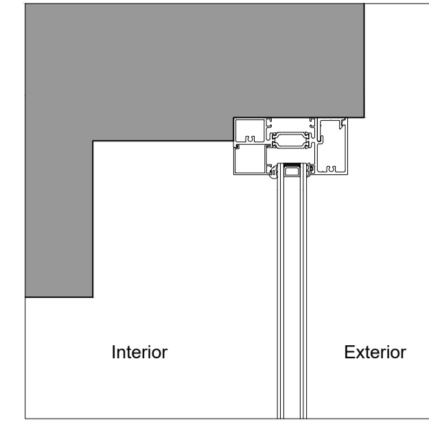
HEAD (SIDE LIGHT)
