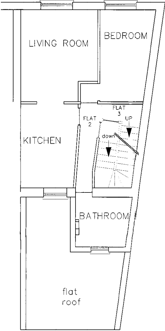
1st Floor 1:100
