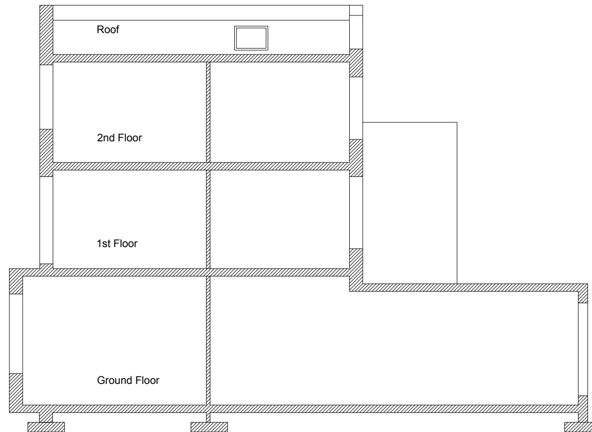
Section 1:100
