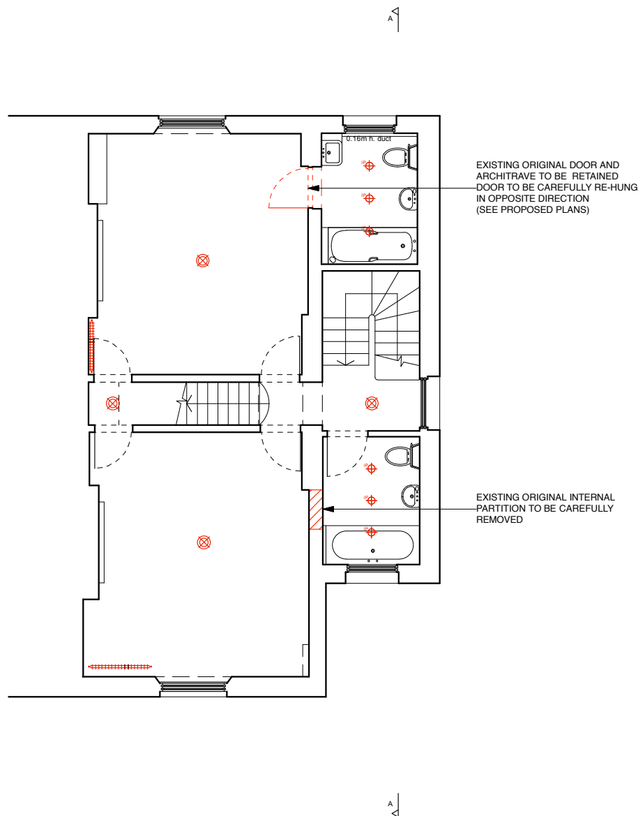
FIRST FLOOR PLAN EXISTING ENABLING WORKS
