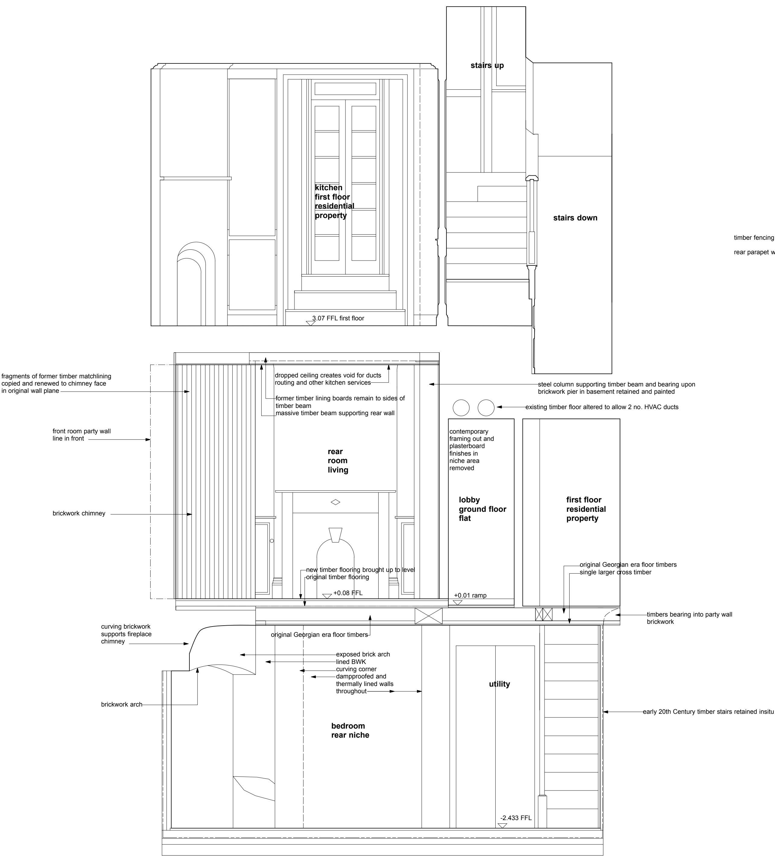
detailed proposed section F-F 1:25
