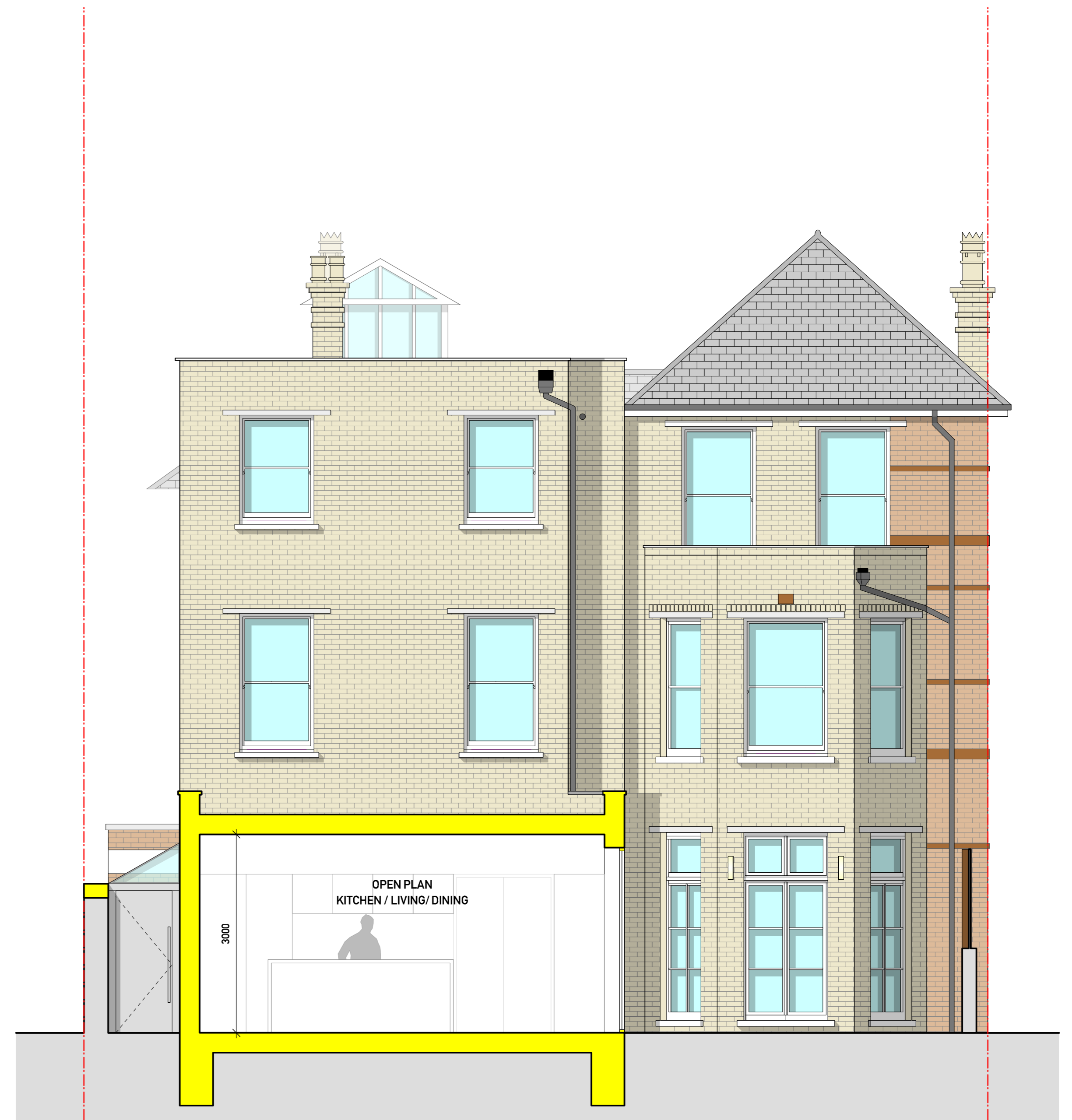
2 Proposed Section B Scale: 1:50
