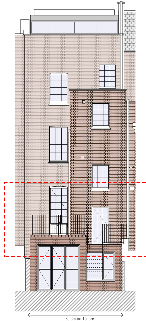
Rear Elevation 1/100
