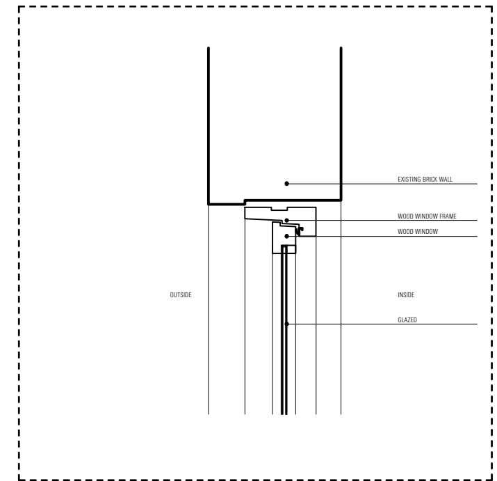
Existing Sill Detail
