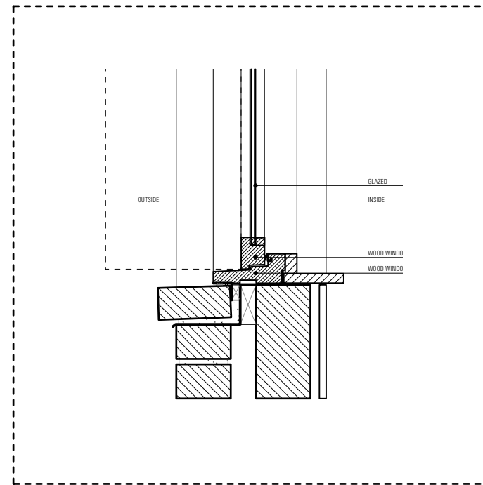
Proposed Head Detail
