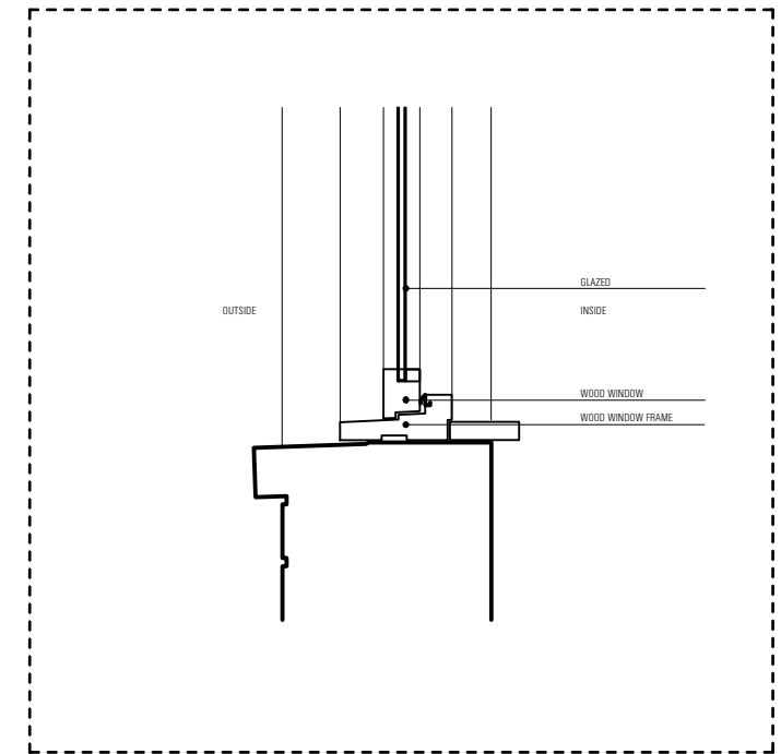
Existing Head Detail
