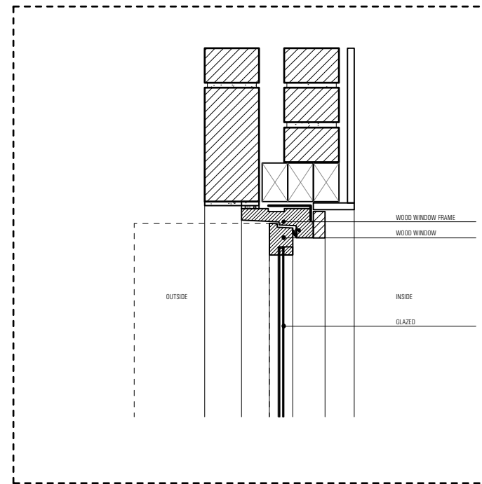
Proposed Sill Detail
