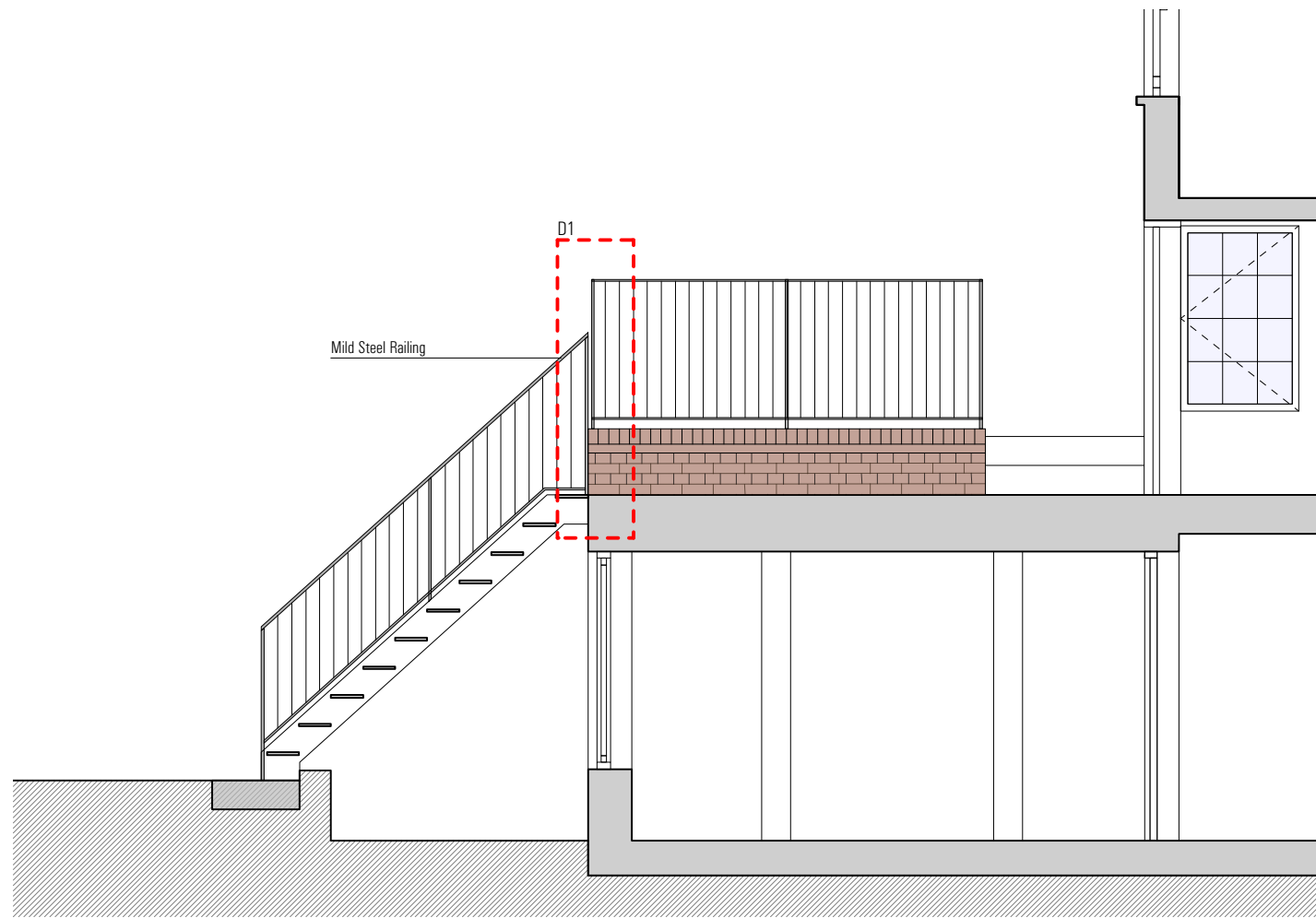
Long Section 1/50
