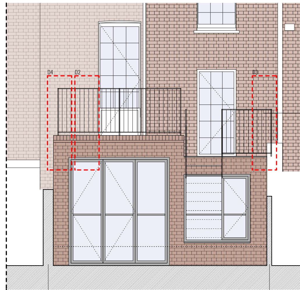
Rear Elevation 1/50
