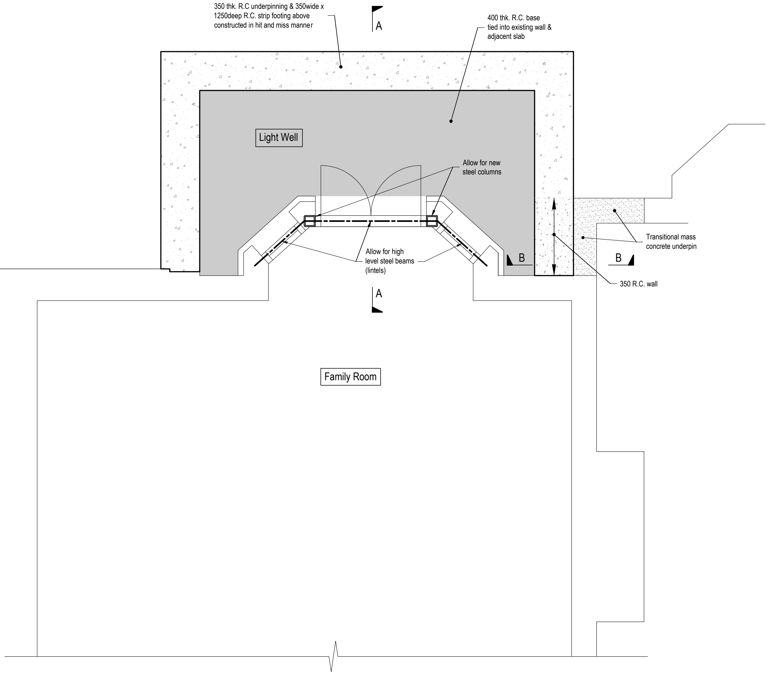
Proposed Partly Lower Ground Floor Scale 1:20
