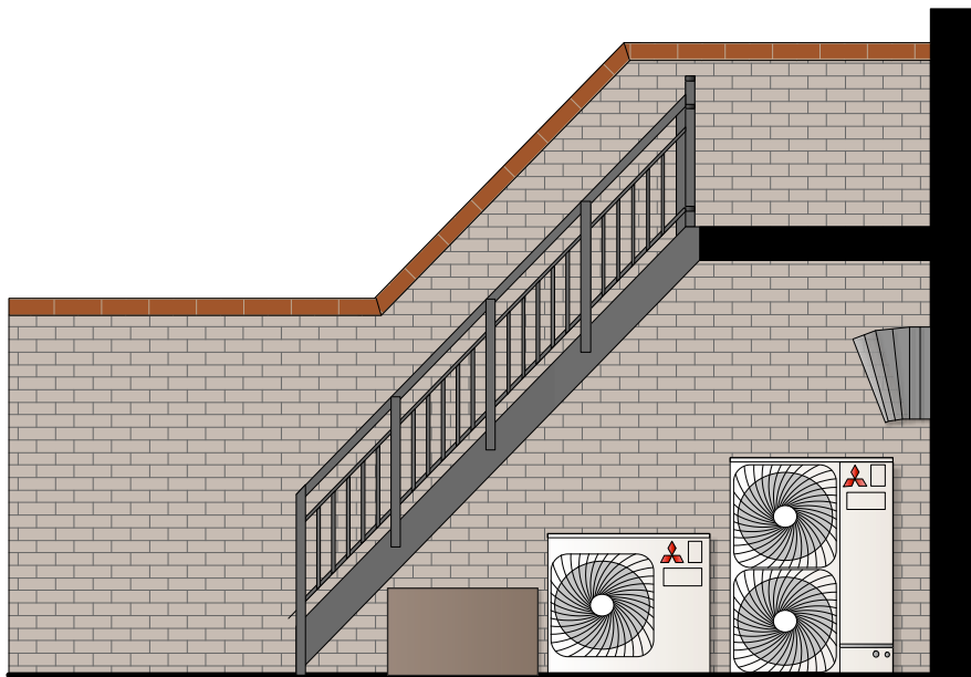
existing HVAC plant equipment elevation BB scale 1:50
