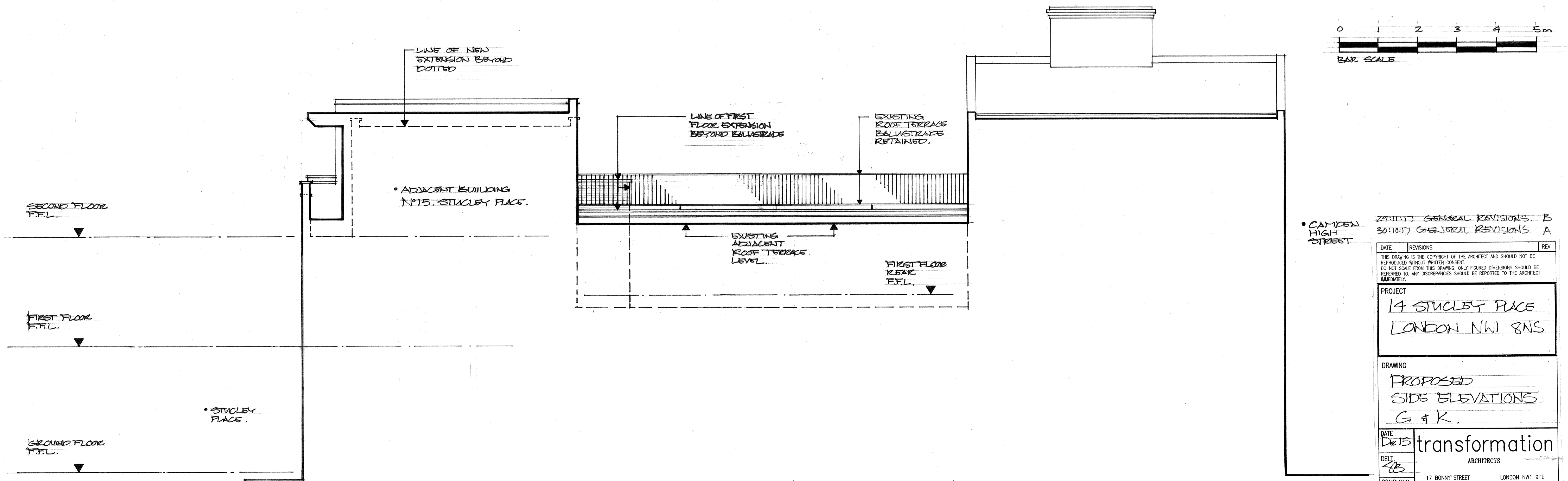
PROPOSED SIDE ELEVATION (G/II)
